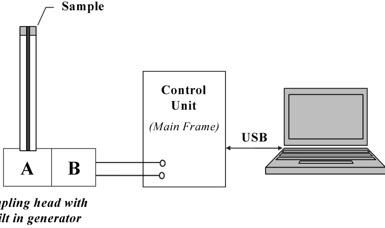
Figure 4. Circuit diagram of a TDS setup. Here A and B are two sampler channels.
