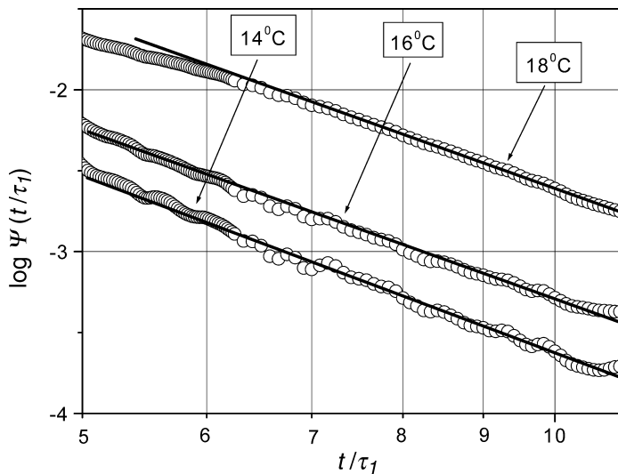
Figure 10. The dipole correlation function \Psi(t/\tau_1) demonstrates power-law behavior for the temperature region near the percolation onset ( T_{\text{on}} = 12^\circ\text{C} ). (Reproduced with permission from Ref. 2. Copyright 2002, Elsevier Science B.V.)
