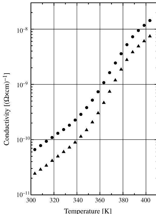
Figure 30. Temperature dependence of the low-frequency conductivity of the 20- \mu\text{m} sample ( \bullet ), and the 30- \mu\text{m} sample ( \blacktriangle ). (Reproduced with permission from Ref. 2. Copyright 2002, Elsevier Science B.V.)
