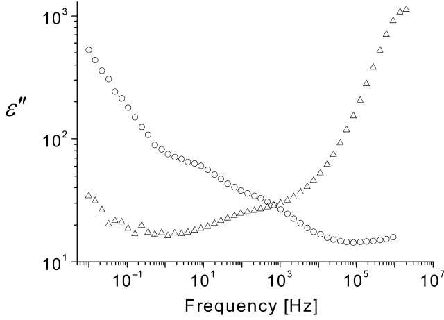
Figure 20. A comparison of the dielectric losses measured at T = 250 K: \triangle represents crystal #1 (KTN doped with Cu ions), and \circ represents crystal #2 (pure KTN). (Reproduced with permission from Ref. 179. Copyright 2004, The American Physical Society.)
