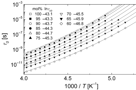
Figure 37. Temperature dependence of \tau_0 obtained by (114) and (115) and representation by the VFT model (full lines) where D and T_v are the same values as those for \tau_{\text{max}} presented in Fig. 26 as well as in the legend (100 to 60 mol%). The pre-exponential factor such as \ln(\tau_{v0}) is shown with the legend.
