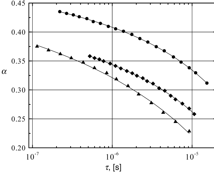
Figure 53. The dependence of \alpha versus relaxation time \tau for QN (●), CN (▲), and MCN (◆) samples. The curves correspond to the model described in this section. (Reproduced with permission from Ref. 2. Copyright 2002, Elsevier Science B.V.)
