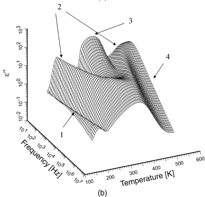
Figure 14. The typical three-dimensional plot of the complex dielectric permittivity real \epsilon' (a) and imaginary part \epsilon'' (b) versus frequency and temperature for porous glass (sample E ). All the details of different sample preparation and their properties are presented in Ref. 156. (Reproduced with permission from Ref. 2. Copyright 2002, Elsevier Science B.V.)
