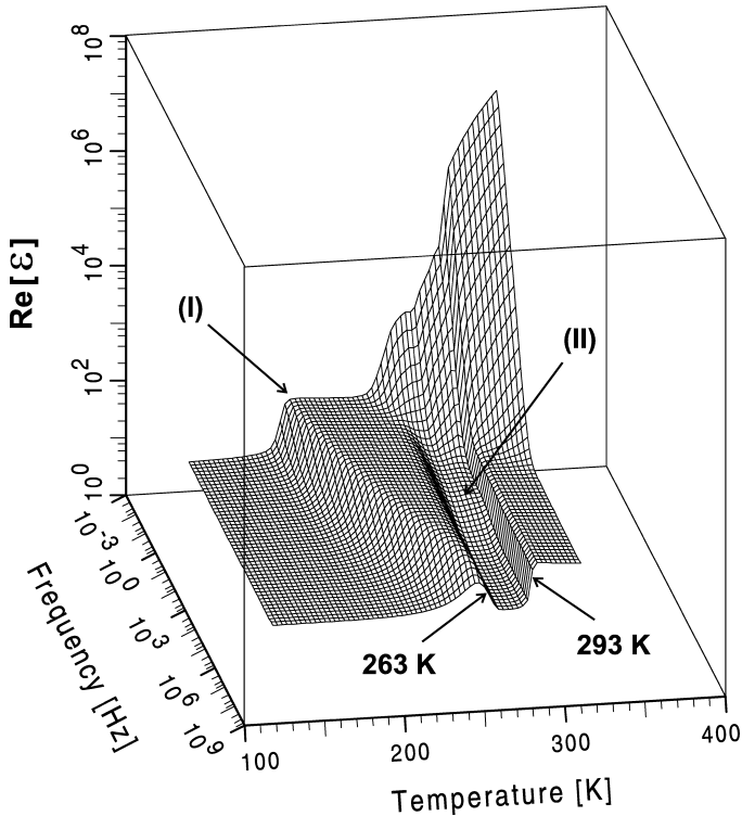
Figure 22. A three-dimensional plot representing the real part of \varepsilon'(\omega) for sample A. The arrows mark the crystallization temperature ( T_x = 263 \text{ K} ), the melting point ( T_m = 293 \text{ K} ), and the principal relaxation process, before (I) and after (II) the crystallization. (Reproduced with permission from Ref. 186. Copyright 2003, The American Physical Society.)
