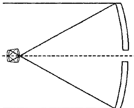
Fig. 1-22. Spherical primary/corrector.
