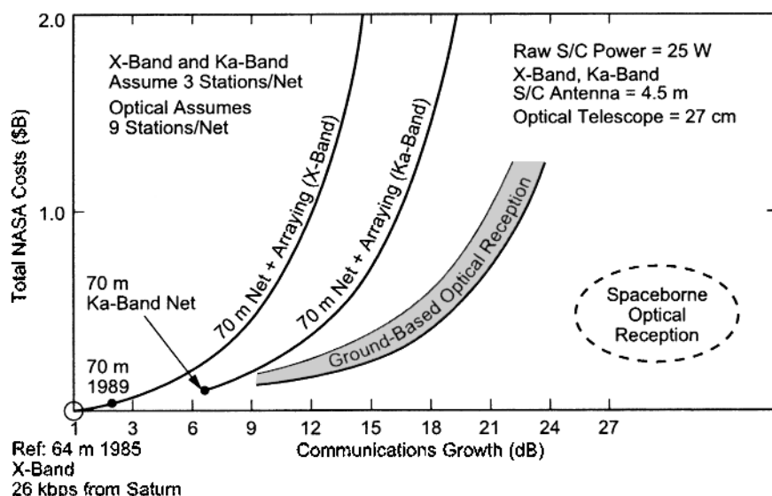
Fig. 1-18. Optimized cost model for Ka-band, X-band, and optical reception.
