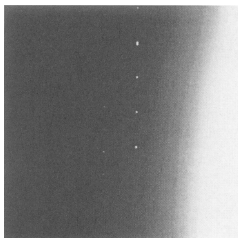
Fig. 1-30. Earth image from Galileo spacecraft showing laser pulses (vertical rows of points).
