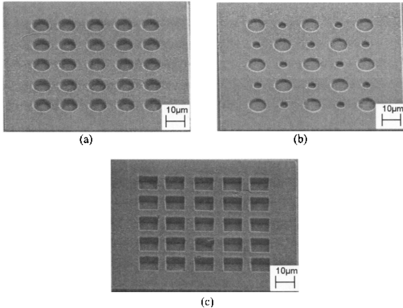
Figure 3. Cavity feature arrays produced on PDMS mold using FIB patterned silicon wafer core: (a) homogeneous round cavity array, (b) heterogeneous round cavity array, and (c) homogeneous square cavity array.
