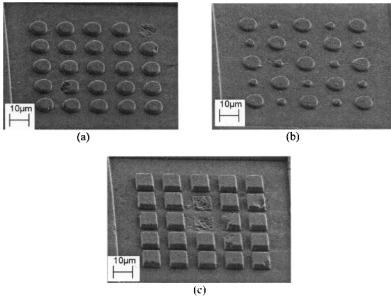
Figure 5. \text{Al}_2\text{O}_3 nanoparticle arrays produced from PDMS mold: (a) homogenous round island array, (b) heterogeneous round island array, and (c) homogenous square island array.
