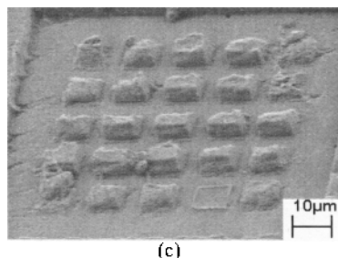
Figure 6. \text{Al}_2\text{O}_3 nanoparticle arrays produced from silicone mold: (a) homogenous round island array, (b) heterogeneous round island array, and (c) homogenous square island array.
