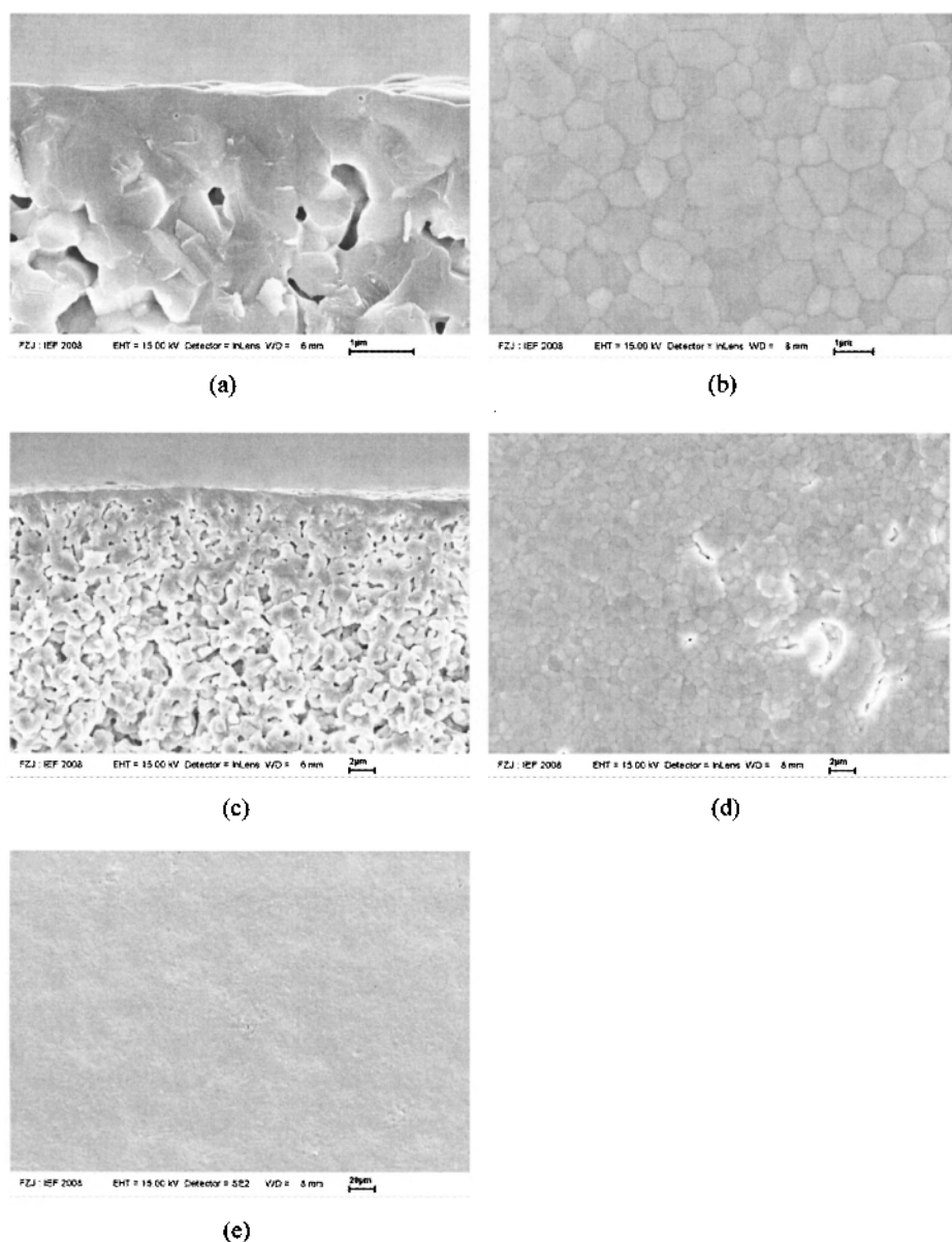
Fig. 9b (a) – (e). Micrographs of the cross-section and surface of the membrane shown in Fig. 8 after firing at 1300°C.
