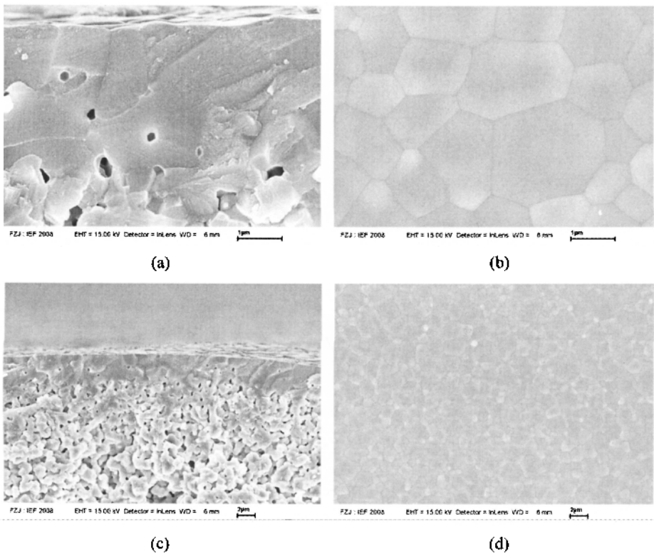
Fig. 10b (a) – (d). Micrographs of the cross-section and surface of the membrane made from the three previously discussed mesoporous membrane layers after firing at 1300°C. (Nano-dispersion 1, Nano-dispersion 2, Colloidal sol: 1 x dip-coating and calcination at 500°C; (a,b) bar = 1 μm, (c,d) bar = 2 μm)
