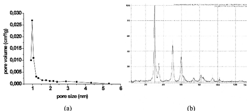
Fig. 12. Pore size distribution (a) and phase structure (b) of the polymeric sol-gel derived material after calcination at 500^\circ\text{C} .
