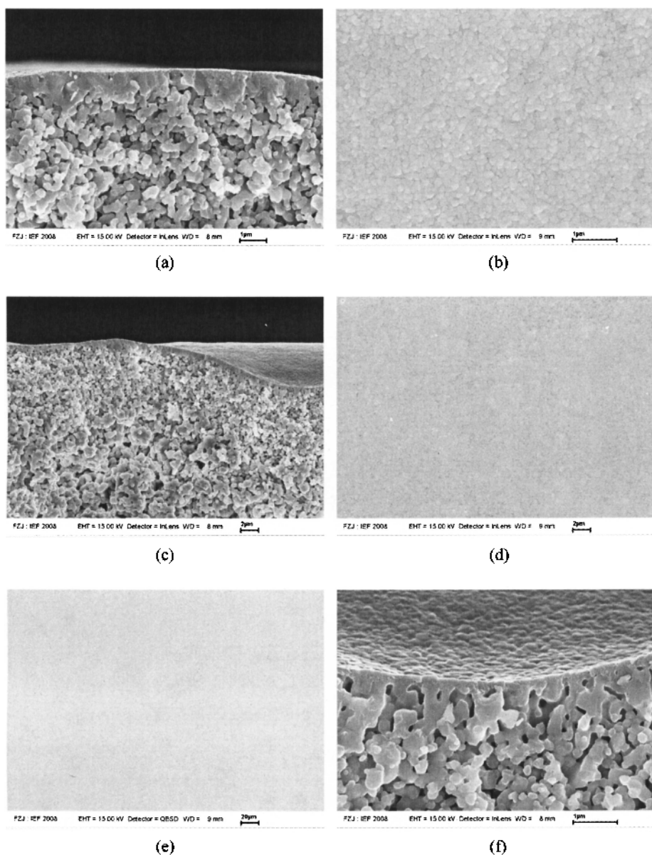
Fig. 13a (a) – (f). Micrographs of the cross-section and surface of the membrane shown in Fig. 11 after firing at 1200°C.
