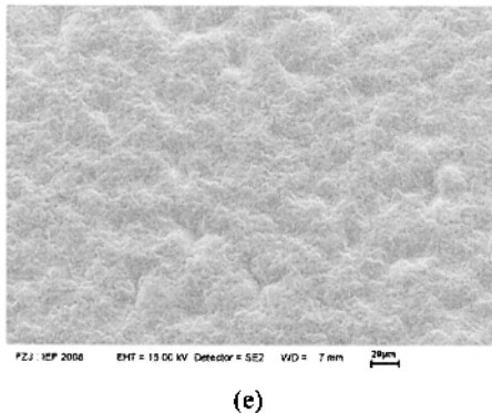
Fig. 10c (e). Micrograph of the surface of the membrane made from the three previously discussed mesoporous layers after firing at 1400°C. (Nano-dispersion 1, Nano-dispersion 2, Colloidal sol: 1 x dip-coating and calcination at 500°C; (e) bar = 20 μm)
