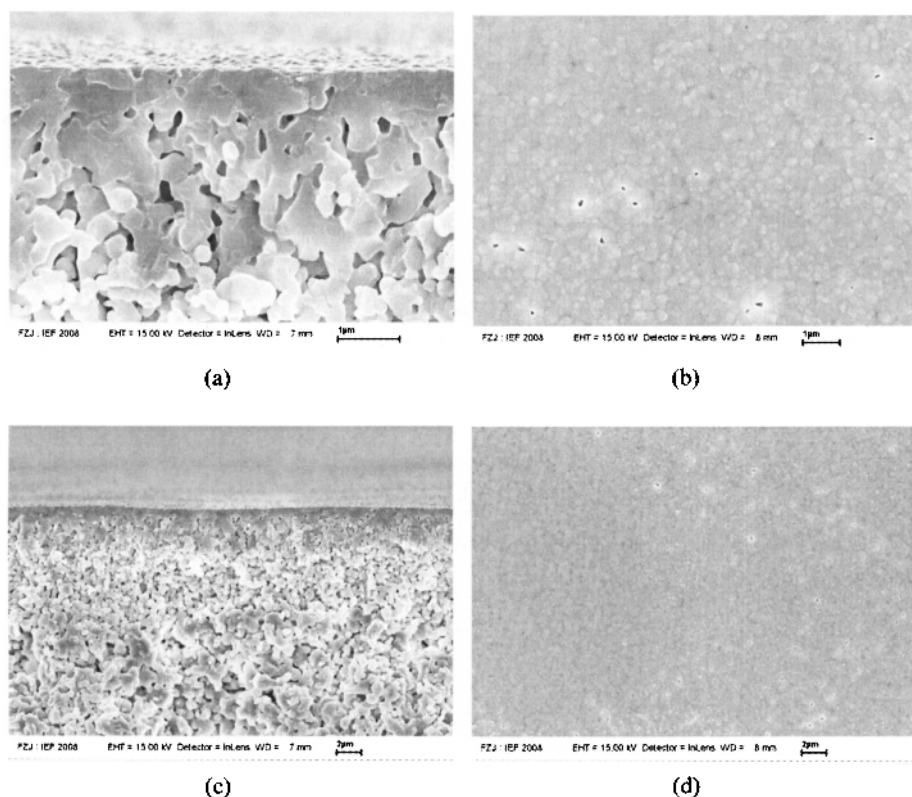
Fig. 10a (a) – (d). Micrographs of the cross-section and surface of the membrane made from the three previously discussed mesoporous membrane layers after firing at 1200°C.
