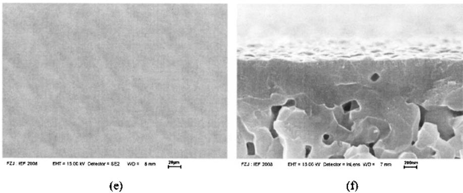
Fig. 10a (e) – (f). Micrographs of the cross-section and surface of the membrane made from the three previously discussed mesoporous layers after firing at 1200°C. (Nano-dispersion 1, Nano-dispersion 2, Colloidal sol: 1 x dip-coating and calcination at 500°C; (e) bar = 20 μm, (f) bar = 200 nm)
