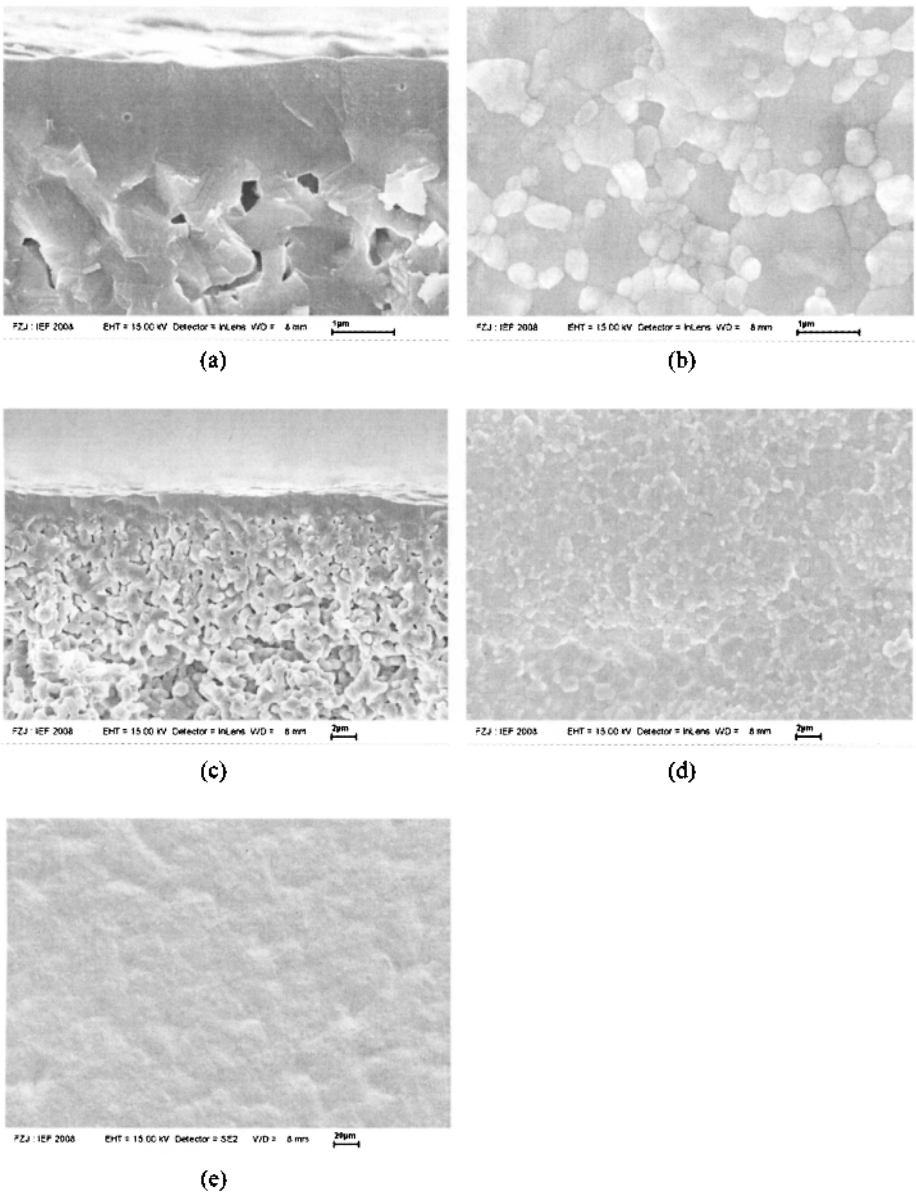
Fig. 13b (a) – (e). Micrographs of the cross-section and surface of the membrane shown in Fig. 11 after firing at 1300°C. (Nano-dispersion 2, Colloidal sol, Polymeric sol: 2 x dip-coating and calcination at 500°C; (a,b) bar = 1 µm, (c,d) bar = 2 µm, (e) bar = 20 µm)
