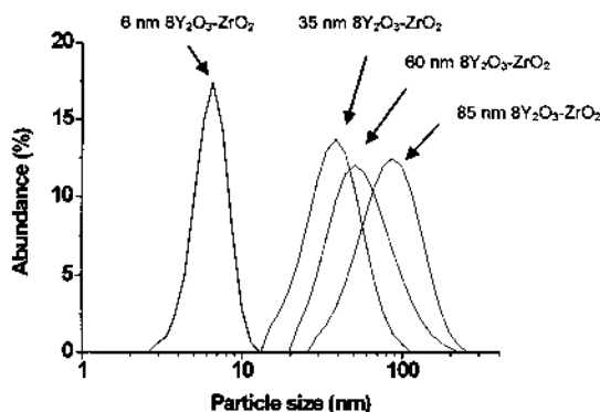
Fig. 3. Particle size distribution of nano-dispersions and sols described in this work
