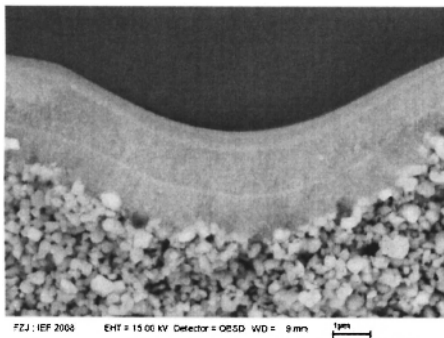
Fig. 11. Overview and detail image of the cross-section of a 8YSZ membrane, obtained by dip-coating subsequently nano-dispersion 2, a colloidal sol and a polymeric sol. (Nano-dispersion 2, Colloidal sol and Polymeric Sol: Layers made by 2 x dip-coating and calcination at 500°C; (a,b) bar = 1 μm)
