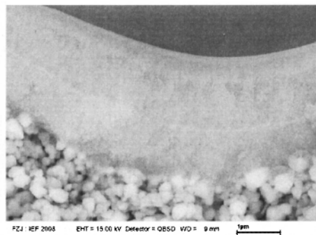
Fig. 11. Overview and detail image of the cross-section of a 8YSZ membrane, obtained by dip-coating subsequently nano-dispersion 2, a colloidal sol and a polymeric sol. (Nano-dispersion 2, Colloidal sol and Polymeric Sol: Layers made by 2 x dip-coating and calcination at 500°C; (a,b) bar = 1 μm)
