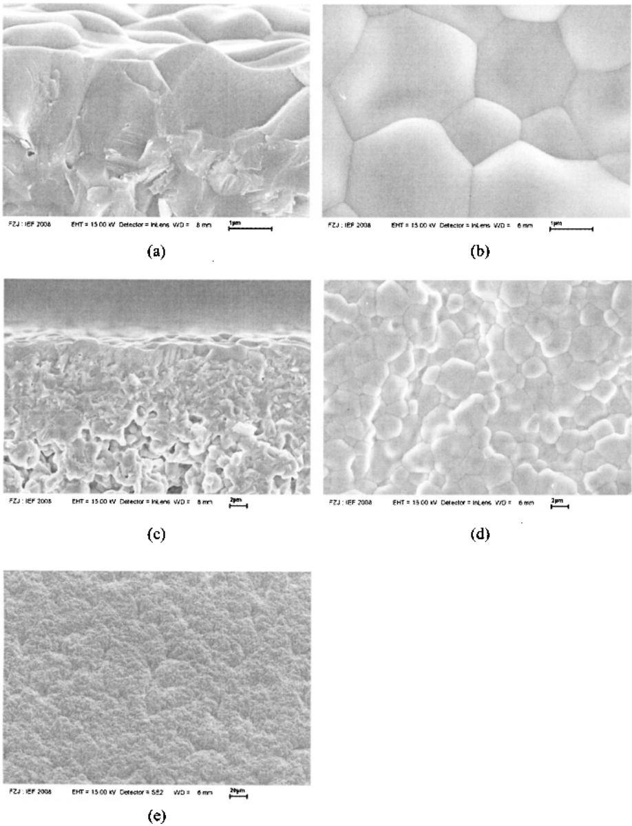
Fig. 13c (a) – (e). Micrographs of the cross-section and surface of the membrane shown in Fig. 11 after firing at 1400°C. (Nano-dispersion 2, Colloidal sol, Polymeric sol: 2 x dip-coating and calcination at 500°C; (a,b) bar = 1 \mu\text{m} , (c,d) bar = 2 \mu\text{m} , (e) bar = 20 \mu\text{m} )
