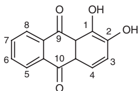
Figure 1.2 Alizarin; 1,2-dihydroxy anthraquinone
