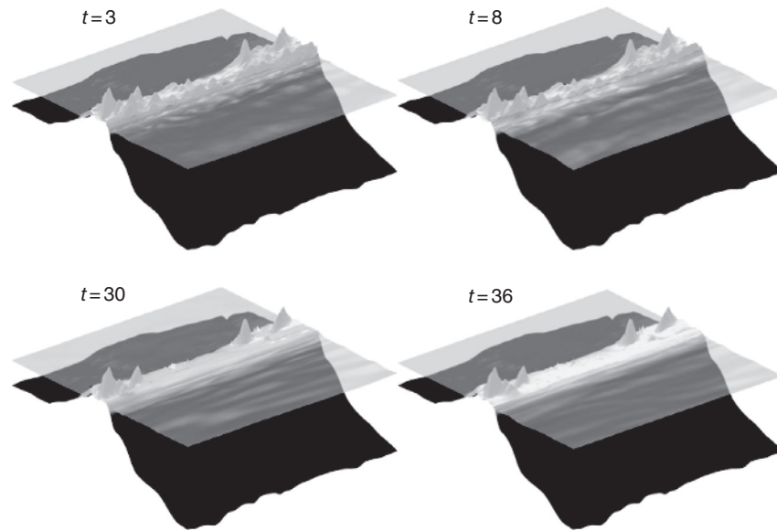
Fig. 1.20 Numerical simulation using the XBeach model of the impact of Hurricane Ivan (the largest of five hurricanes to strike to US coast in 2004) on a 2-km wide section of Santa Rosa Island, a narrow barrier island in Florida. The Gulf of Mexico is in the lower right and the back barrier bay in the upper left of all four panels. The simulation was run over 36 hours and the four panels represent the water-level variation and barrier morphology at different time steps. The maximum storm surge and significant wave height used for forcing the model were 1.75 m and 7 m, respectively, and were attained at t = 18 hours. Note the extensive overwashing at t = 30 hours and the complete destruction of the dunes in the central part of the modelled region. (Source: McCall et al. 2010. Reproduced with permission of Elsevier.) For colour details, please see Plate 4.
