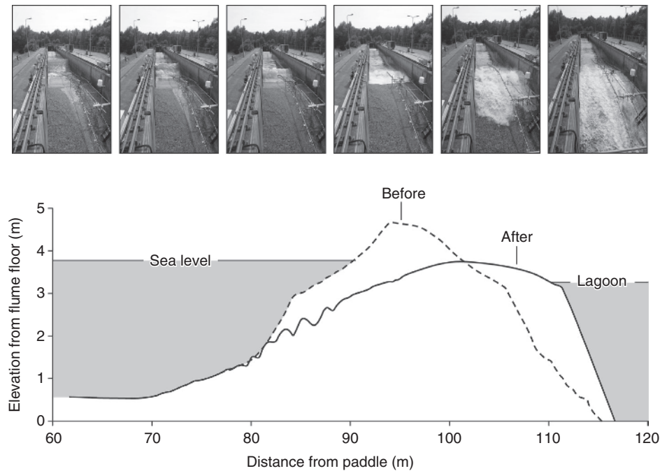
Fig. 1.21 Physical simulation of overwash on a gravel barrier constructed in the Delta Flume, The Netherlands, during the BARDEX experiment. (Source: Williams et al. 2012. Reproduced with permission of Elsevier.) The sequence of photos in the top panels represents the various stages of wave transformation of one of the overwashing waves. The bottom panel shows the morphological change after 2.5 hours of exposure to overwash, characterized by a lowering of the barrier crest by about 1 m and the development of an extensive washover deposit at the back of the barrier. The wave conditions during this test were characterized by a significant wave height of 0.8 m and a peak wave period of 8 s.
