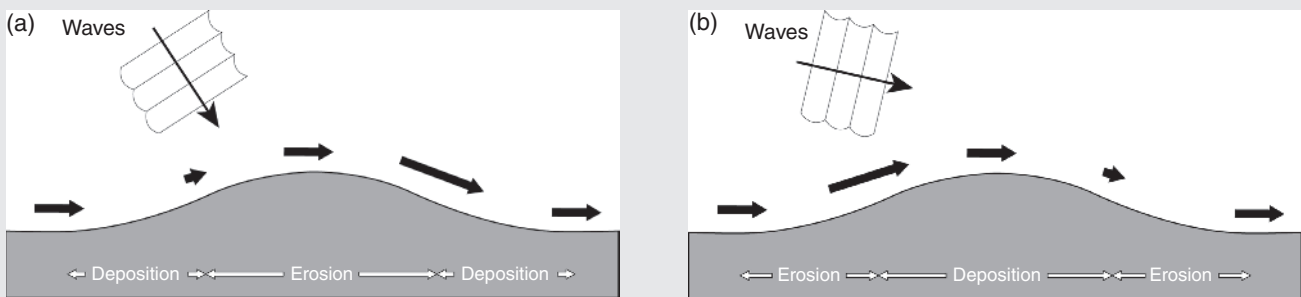
Fig. 1.11 Schematic illustrations of shoreline change caused by high-angle and low-angle waves. When the angle between the deep-water wave crests and the shoreline is less than the flux-maximizing angle ( <45^\circ ) shoreline perturbations will be smoothed out, whereas for angles greater than the flux-maximizing angle ( >45^\circ ) the perturbations will grow. (Source: Adapted from Coco and Murray 2007. Reproduced with permission of Elsevier.)
