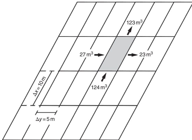
Fig. 1.19 Schematic illustrating the use of the sediment continuity equation for grid-based numerical models. See text for explanation.
