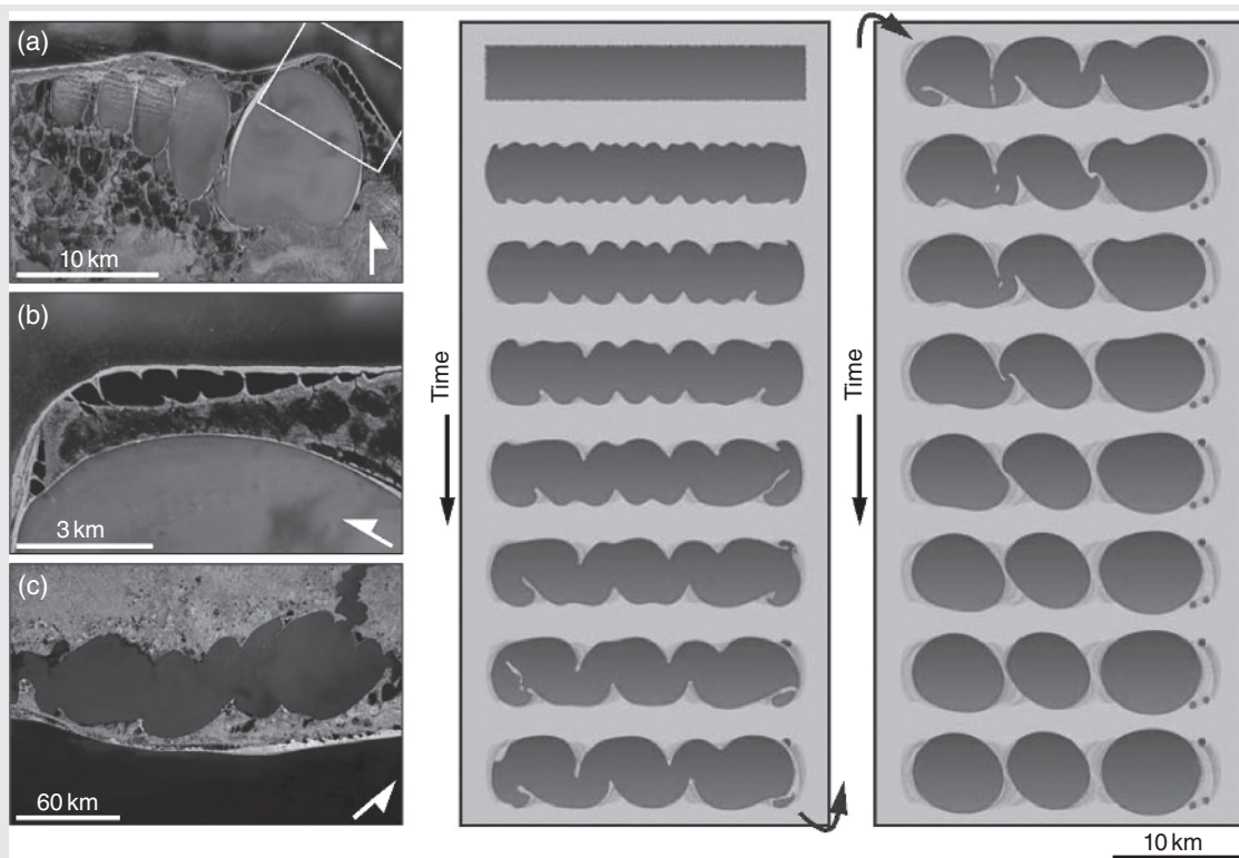
Fig. 1.10 Natural examples of enclosed water bodies with cusped features and segmented water bodies. (a) Laguna Val'karkynmangkak, Russia; (b) inset of (a); and (c) Lagoa Dos Patos, Brazil. The results of a numerical simulation of the formation of cusped features and segmented water bodies are shown in the right panels. (Source: Ashton et al. 2009. Reproduced with permission of the Geological Society of America.) For colour details, please see Plate 2.
