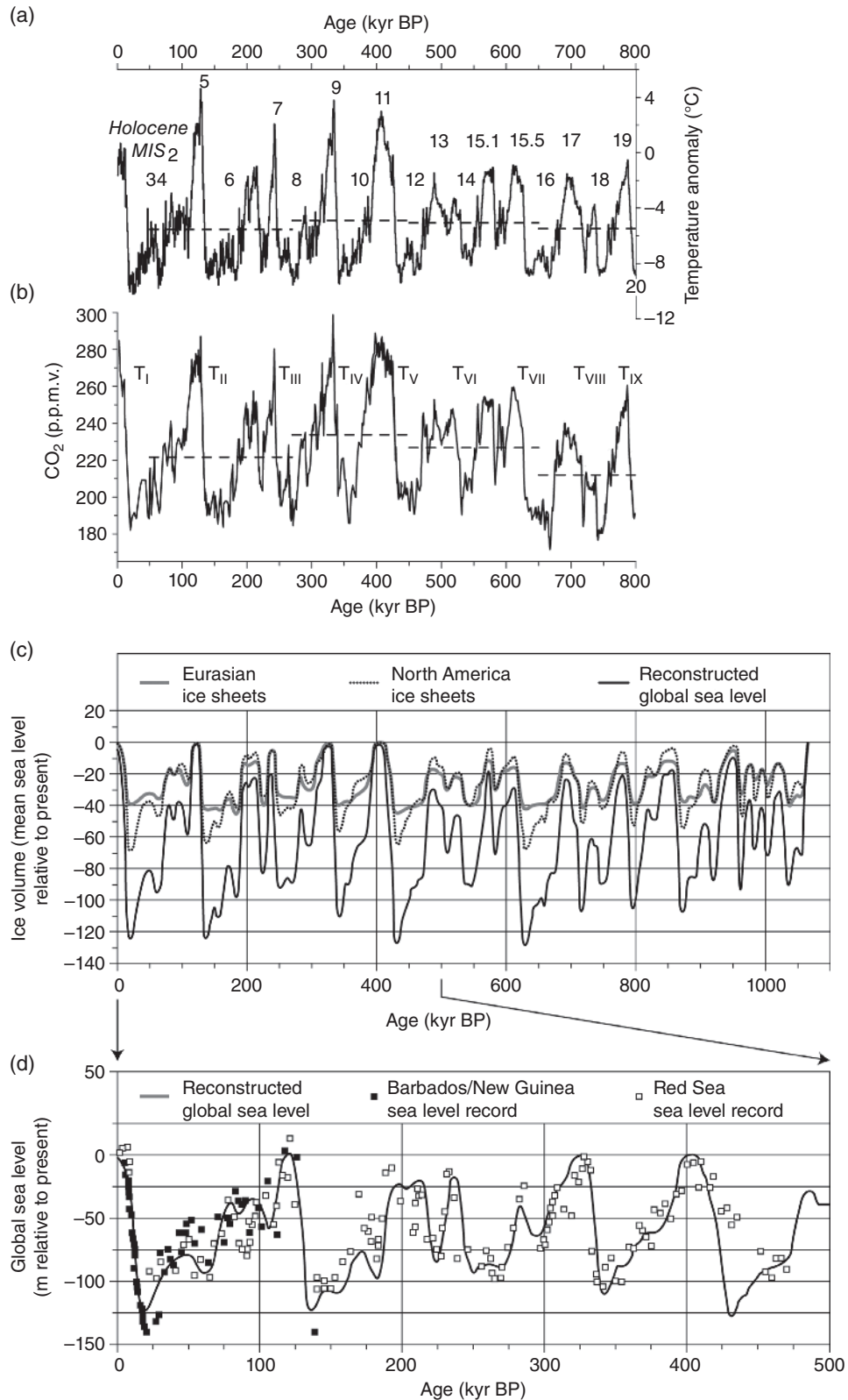
Fig. 1.13 Temperature (a) and carbon dioxide record (b) from Antarctica. (Source: Lüthi et al. 2008. Reproduced with permission of Nature Publishing Group.) (c) Modelled global sea-level record for the past 1M years, with contributions from Eurasian and North American ice sheets (Source: Bitanja et al. 2005). In (d), the model output is compared with the longest Quaternary sea-level record in the world, the record from the Red Sea (Source: Siddall et al. 2003), and with coral reef data from Barbados and New Guinea (Source: Lambneck and Chappell 2011).
