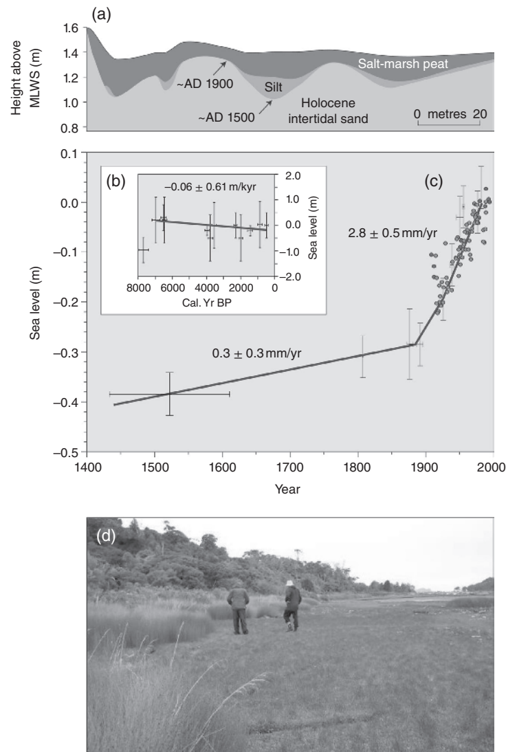
Fig. 1.12 Deriving sea-level history from salt-marsh stratigraphy. (a) Stratigraphy of a salt marsh in southern New Zealand. The marsh developed in the past half millennium on a substrate of late Holocene intertidal sands. The sands were deposited in the middle and late Holocene when sea level was slightly higher than present. MLWS, mean low water spring. (b) Since about AD 1900, accumulation has been very rapid as a consequence of the accommodation space provided by the sharp sea-level acceleration (c). The crosses in (b) and (c) represent dated samples of shells and plant material, respectively, which can be related to former sea levels (with vertical and age uncertainties). Different coloured dots in (c) represent annual measurements of sea level from two nearby tide gauges. Cal. Yr BP, calibrated years before present. (d) The photo shows an overview of the marsh, which can be found on the Catlins coast in southeastern New Zealand, near the village of Pounaweia. (Source: Adapted from Gehrels et al. 2008. Reproduced with permission of John Wiley & Sons.) For colour details, please see Plate 3.
