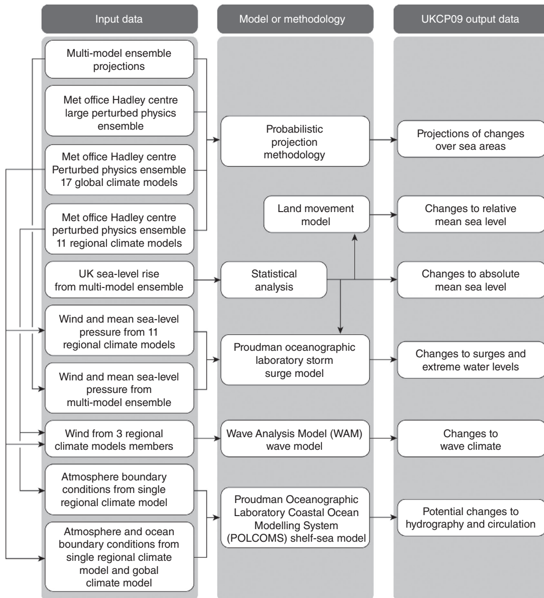
Fig. 1.15 Example of a regional approach to predicting sea-level changes. UKCP09, United Kingdom Climate Projections 2009. (Source: Adapted from Lowe et al. 2009. © UK Climate Projections, 2009.)
