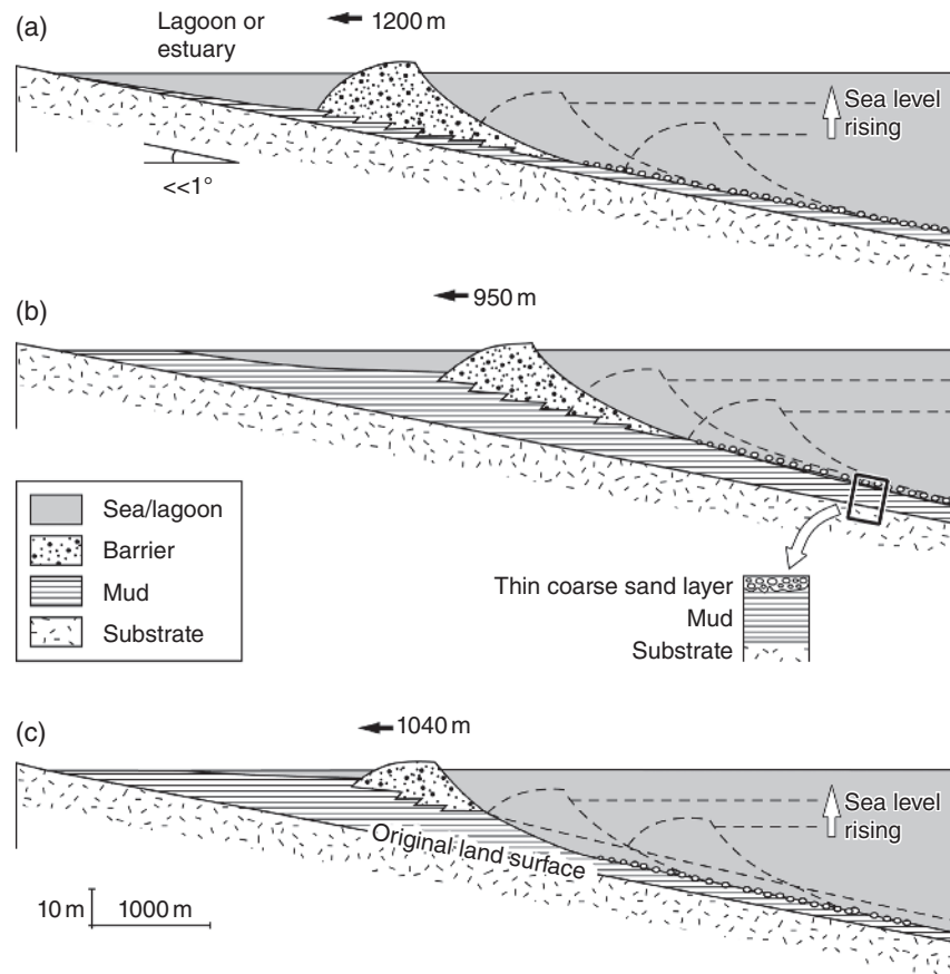
Fig. 1.18 Example of output of the Shoreline Translation Model (STM) of Cowell et al. (1995) showing the response of a barrier to sea-level rise. In Case (a), a small amount of mud deposition in the back barrier lagoon has little effect on barrier size or coastal behaviour, but with mud accumulating almost as fast as sea level is rising, as in Case (b), the barrier decreases in size and recession slows down. In Case (c), a deficit in the nearshore sediment budget, for example induced by a negative littoral drift differential, is superimposed on Case (b), resulting in a reduction in the size of the barrier and an increase in the recession rate. In addition to showing the different stages of barrier recession, the model also reproduces the stratigraphy, and in all cases lagoonal muds conformably blanket the substrate beneath and to the seaward of the barrier; after the barrier passes, wave reworking ensures that the bed is soon veneered by a coarse lag. (Source: Roy et al. 1994. Reproduced with permission of Cambridge University Press.)
