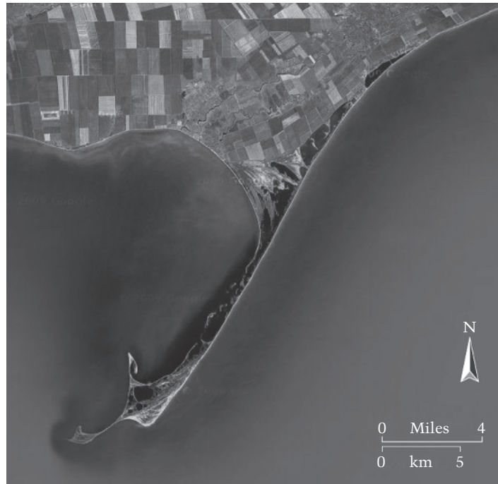
Fig. 1.9 Flying spit in the Sea of Azov, Ukraine. The formation of these features has intrigued coastal scientists for decades, but numerical modelling by Ashton and Murray (2006a, b), based on the relation between the longshore sediment transport rate and the deep-water wave angle (see Box 1.1), seems to have provided a satisfactory explanation for their formation. (Source: Image © 2013 Terrametrics. Map data © 2013 Google.)
