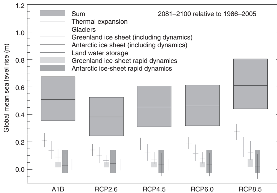
Fig. 1.14 Projections from process-based models with likely ranges and median values for global mean sea-level rise and its contributions in 2081–2100 relative to 1986–2005 for the four RCP scenarios and scenario SRES A1B used in the AR4. From Church et al. (2014). (Source: Meehl et al. 2007. Reproduced with permission of the IPCC.)
