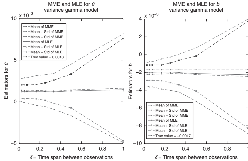
FIGURE 1.3 Sampling mean and standard error of the MME and MLE for the parameters \theta and b based on 200 simulations with values T = 252, \sigma = 0.0127; \kappa = 0.2873; \theta = 1.3 \times 10^{-3}; b = -1.7 \times 10^{-3} .
