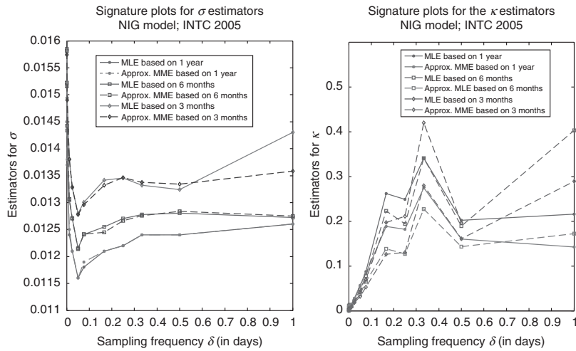
FIGURE 1.6 Signature plots for the MLE and MME for \sigma under a NIG model based on different time horizons.
