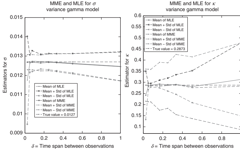
FIGURE 1.2 Sampling mean and standard error of the MME and MLE for the parameters \sigma and \kappa based on 200 simulations with values T = 252 , \sigma = 0.0127 ; \kappa = 0.2873 ; \theta = 1.3 \times 10^{-3} ; b = -1.7 \times 10^{-3} .
