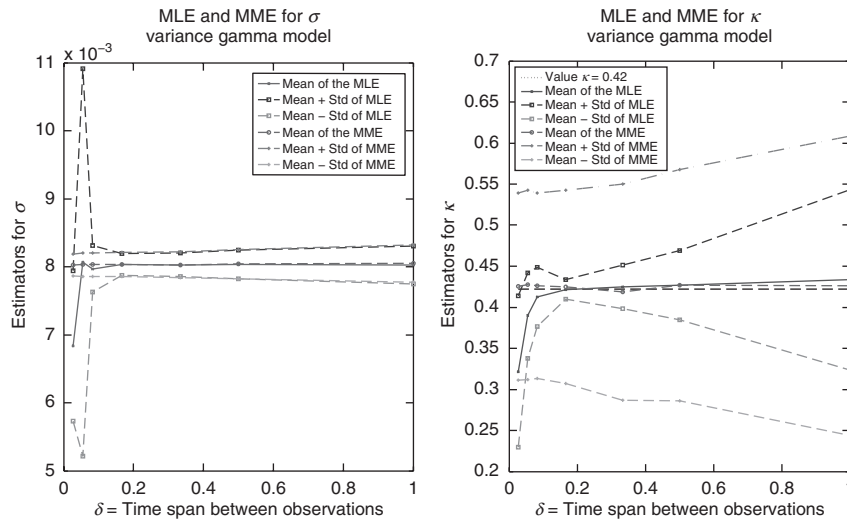
FIGURE 1.1 Sampling mean and standard error of the MME and MLE for the parameters \sigma and \kappa based on 100 simulations of the VG model with values T = 252 * 3, \sigma = \sqrt{6.447 * 10^{-5}} = 0.0080; \kappa = 0.422; \theta = -1.5 * 10^{-4}; b = 2.5750 * 10^{-4}.
