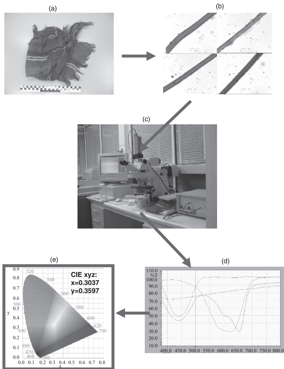
Figure 1.8 Principles of the determination of colour by the MSP-DAD technique – an example of fibres analysis: (a) textile sample; (b) fibre samples; (c) MSP-DAD set; (d) examples of spectra; (e) illustration of concepts of CIE xyz systems and an example of calculated chromaticity coordinates obtained for a fibre sample ( x + y + z = 1 ).
