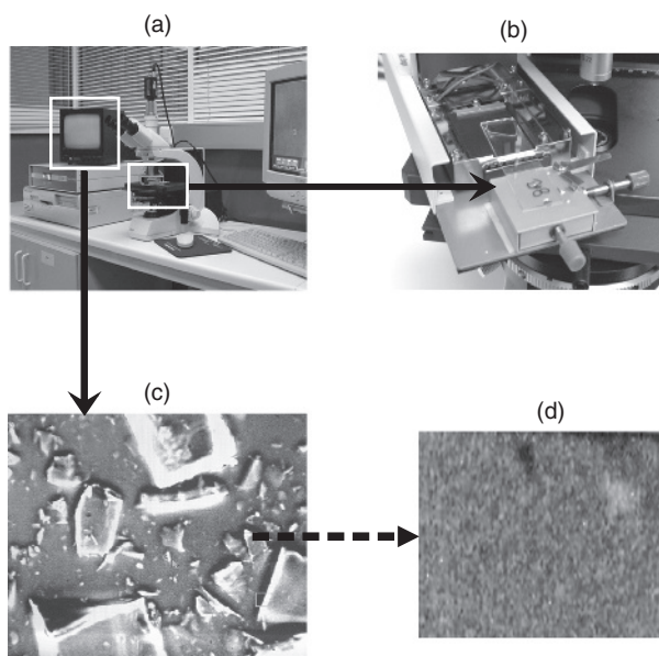
Figure 1.3 Principles of the thermoimmersion method for determination of the refractive index of glass microtraces: (a) GRIM2 set; (b) the appearance of a glass sample in an immersion oil on a microscopic slide located at the hot stage; (c) an image of glass edges in an immersion oil at the temperature when its refractive index is different from the refractive index of the measured glass sample; (d) an image of glass edges in an immersion oil at a matching temperature when its refractive index is equal to the refractive index of the measured glass sample.
