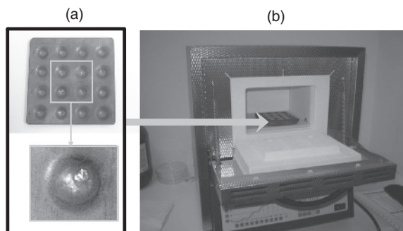
Figure 1.4 Annealing of glass fragments: (a) a metal holder containing glass fragments prepared for annealing; (b) a Nabertherm L3/11 muffle furnace with P320 programmer.
