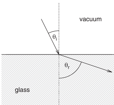
Figure 1.2 Refraction of light when passing from vacuum to glass.
