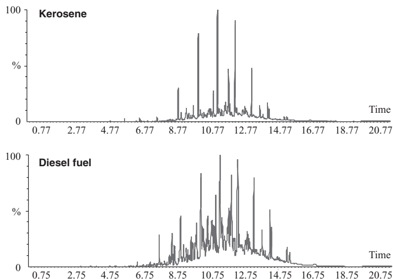
Figure 1.6 Chromatograms of partially evaporated samples of kerosene and diesel fuel revealing similarities in their composition.
