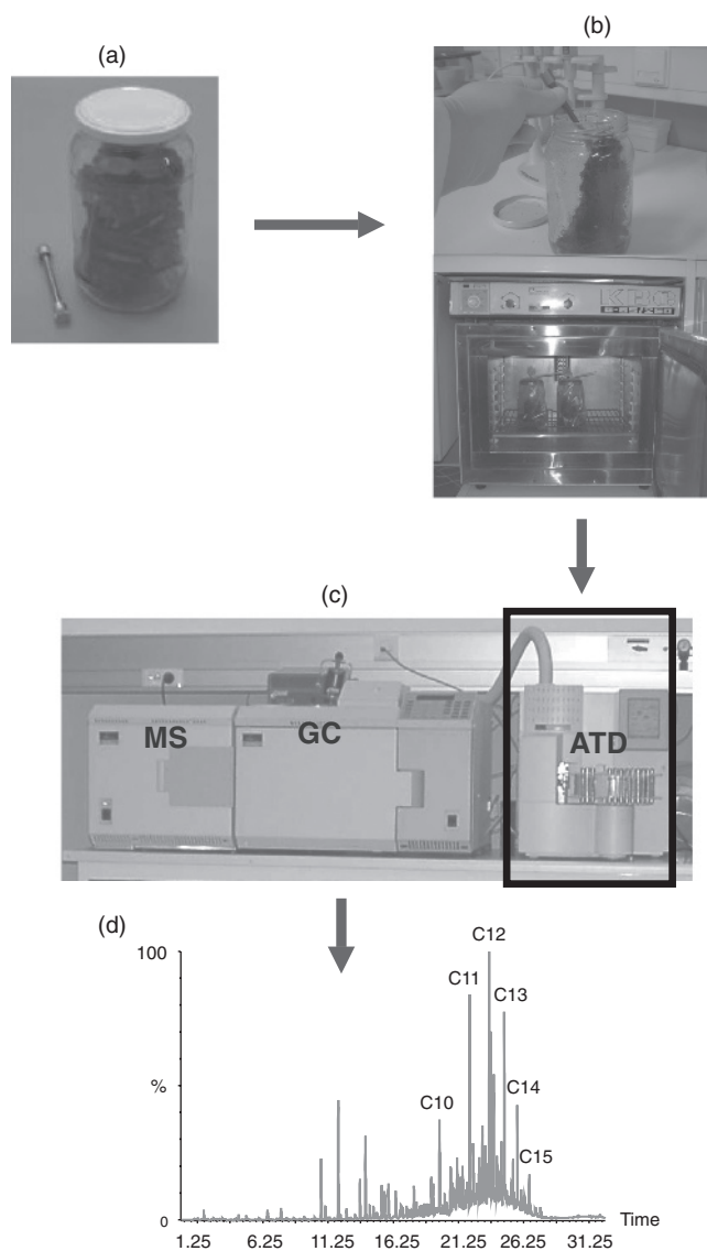
Figure 1.5 Principles of analysis of fire debris by the ATD-GC/MS technique: (a) a sample collected at the scene of a fire; (b) a metal tube filled with adsorbent Tenax TA™ is placed in a jar with fire debris (top) and the jar put in an oven at a pre-concentration stage of analysis (bottom); (c) the metal tube is placed in the automatic thermal desorber (ATD; black box) and the sample analysed by the GC/MS technique; (d) a chromatogram, showing a result that allows the investigator to determine the category (here: kerosene) from which the flammable liquid originates.
