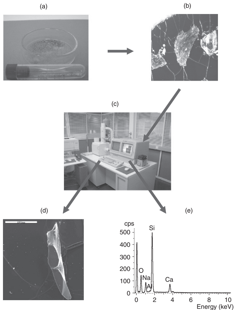
Figure 1.1 Principles of determination of elemental composition of glass fragments by the SEM-EDX technique: (a) debris collected from suspect clothes; (b) glass fragments located on an SEM stub; (c) view of SEM-EDX equipment; (d) SEM image of an analysed glass sample; (e) the spectrum of a glass sample obtained from an EDX detector.
