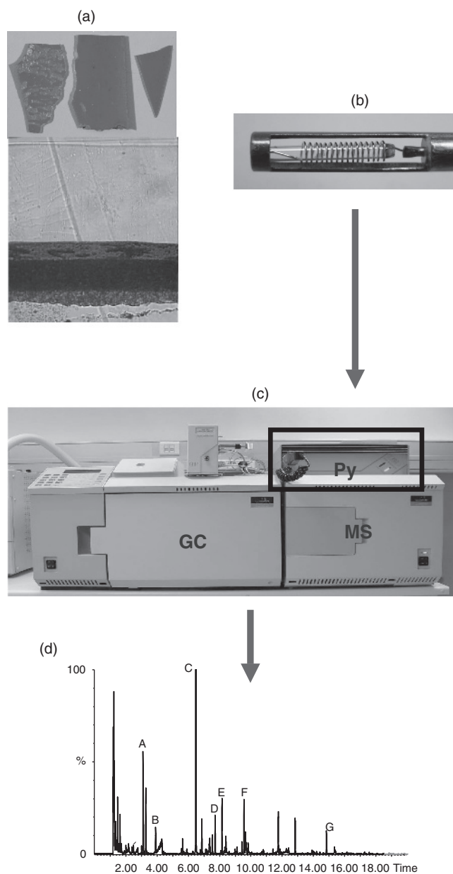
Figure 1.7 Principles of the analysis of car paints by the Py-GC/MS technique: (a) an image of a sample collected at the scene of a car accident (top) and a cross-section of car paint (bottom); (b) a car paint sample (50–100 \mu\text{g} ) put into a quartz tube located in the platinum coil of a CDS Pyroprobe 2000 pyrolyser (Py); (c) an analysis of pyrolysis products by GC/MS; (d) an example of a chromatogram obtained for styrene-acrylic-urethane car paint.
