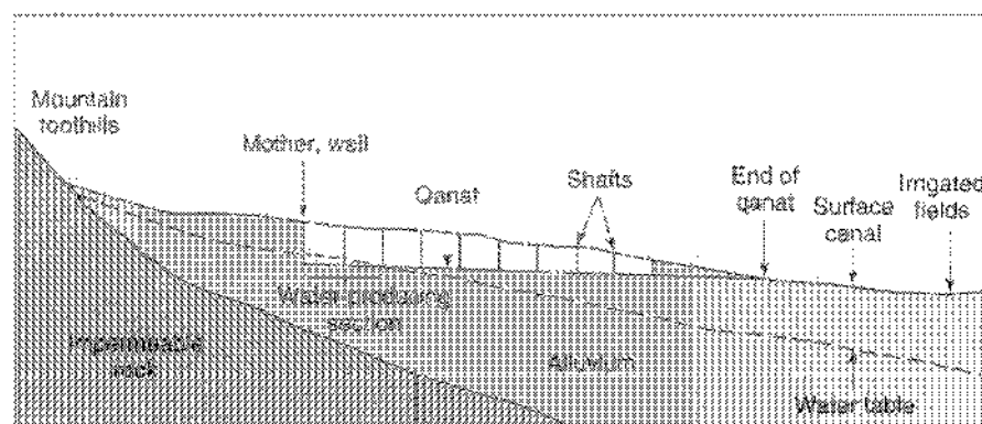
Figure 1.2.1. Vertical cross section along a qanat (after Beaumont 12 ).
