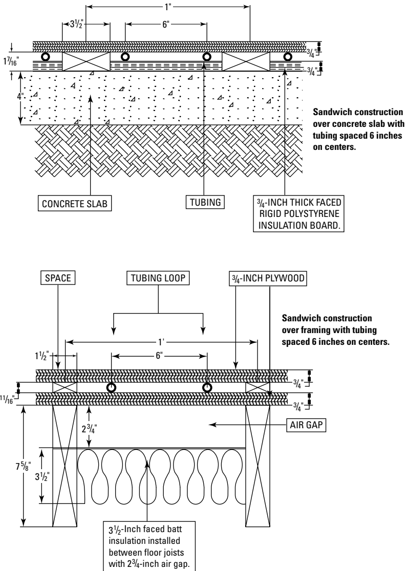
Figure I-24 Examples of sandwich floor construction.
