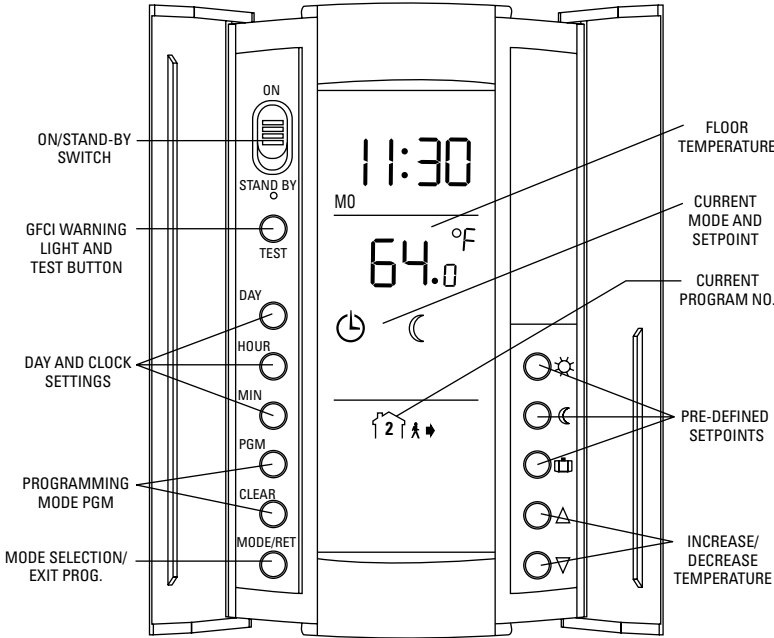
Figure 1-34 Programmable thermostat with digital display for an electric radiant floor heating system. (Courtesy Watts Radiant, Inc.)
