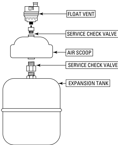
Figure I-18 Air separator and expansion tank.
