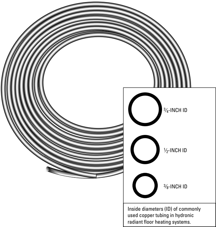
Figure 1-4 Copper tubing.
