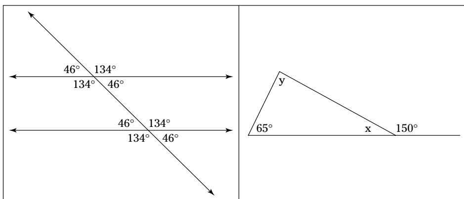
Figure 1-2: Parallel lines with a transversal and a trian- gle with an exterior angle.
