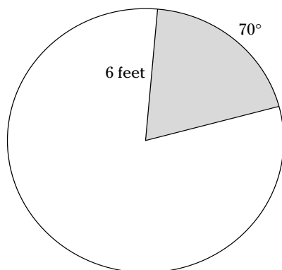
Figure 1-3: A sector of a circle.
