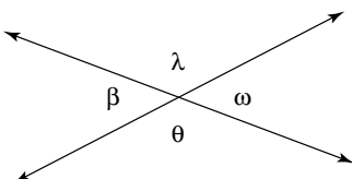
Figure 1-1: Two intersecting lines form four angles.
