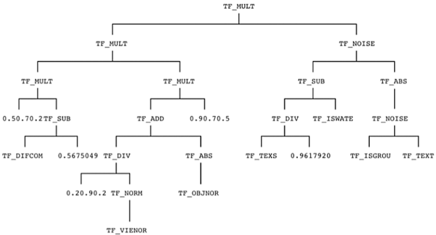
Figure 1.20 An (incomplete) example shader tree and compiled script.
