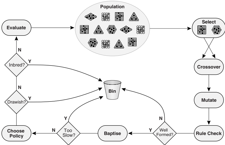
Figure 1.12 Game life cycle (from [10]).
