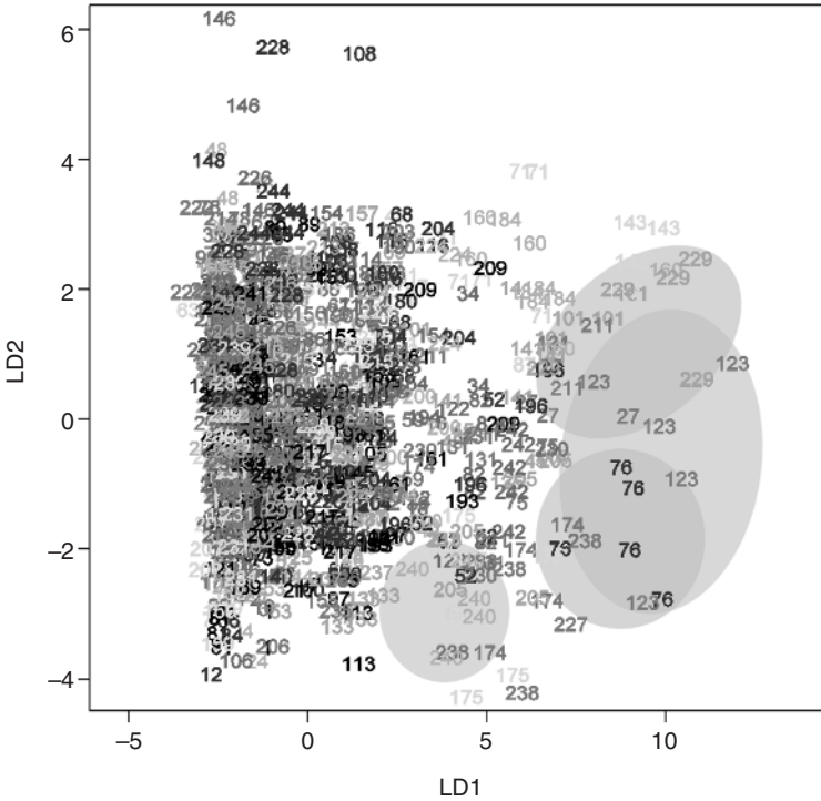
Figure 1.5 LDA-transformed space of metrics recorded in Pac-Man . Each number represents a player, and each number will appear five times, its position marking the coordinates of the feature vector defined by one session of that player. Some player sessions have been highlighted by shaded circles. (Reproduced from [6].)
