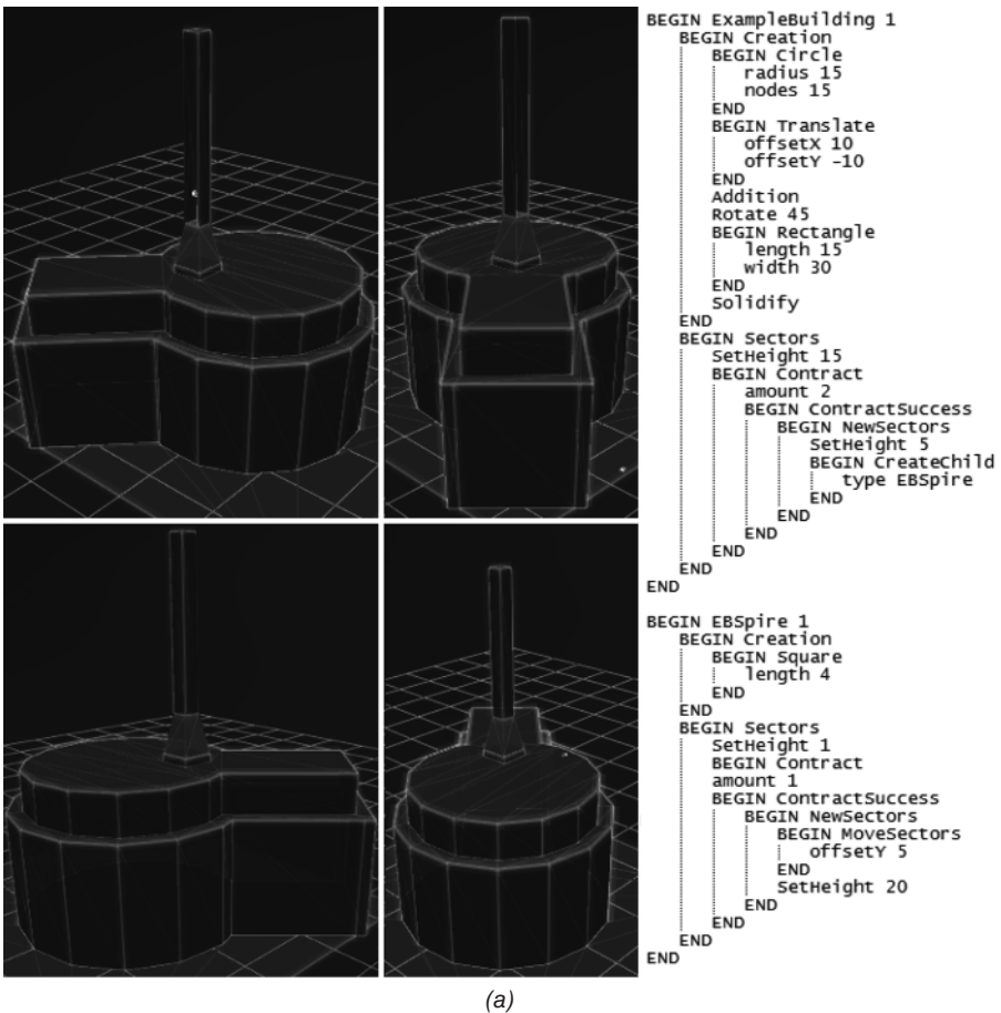
Figure 1.23 (a) Example building along with script responsible for its generation.
