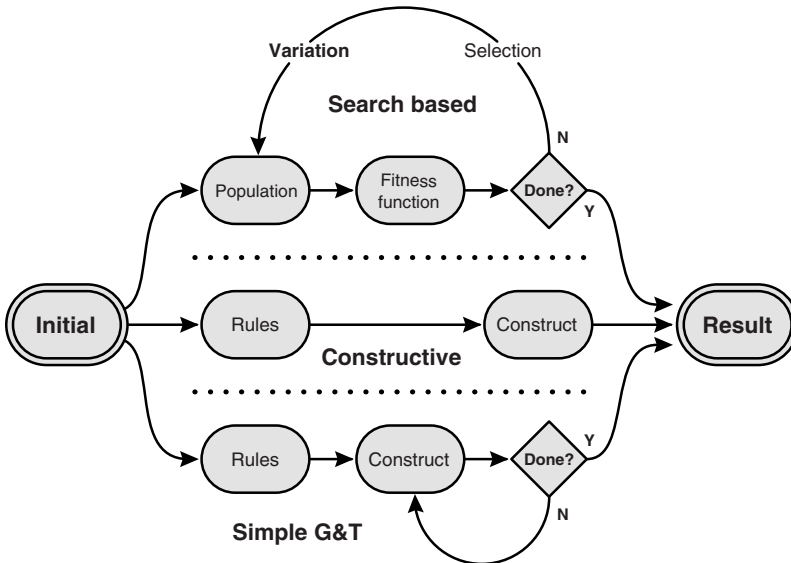
Figure 1.2 Main forms of PCG (from [58]).
