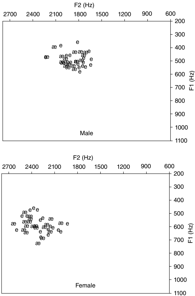
Figure 1.1 Formant plot of 'ㅐ' and 'ㅓ' (i.e. /e/ and /æ/).
