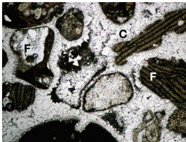
Figure 1.5 Thin-section image of a Bermuda Pleistocene limestone composed of biofragments (F) and interparticle cement (C), image width 1 cm.
