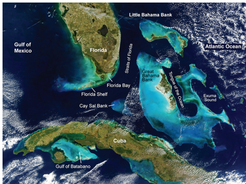
Figure 1.7 A satellite view of southern Florida, Cuba, and the Bahama Banks. The light blue areas, mostly <5 m deep, are regions of carbonate sediment formation. Source: Jones (2010). Reproduced with permission of the Geological Association of Canada.
