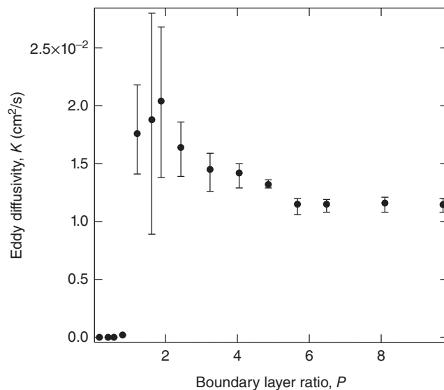
Figure 1.24. Dependence of eddy diffusivity for quasi-geostrophic potential vorticity on boundary layer ratio \mathcal{P} (proportional to \Omega ) derived using data from correlating (u'q') against \partial\bar{q}/\partial r in the rotating annulus model simulations of Pérez et al. [2010].
