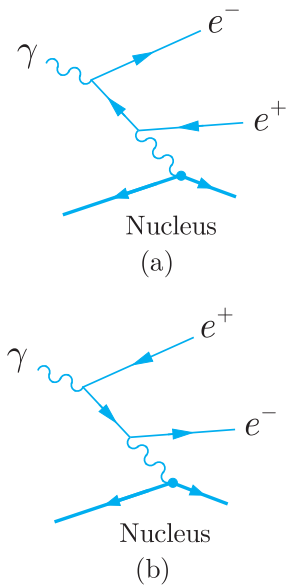
Figure 1.11 The pair production process \gamma + (Z, A) \rightarrow e^+ + e^- + (Z, A) in lowest order. The two diagrams represent ‘distinct’ contributions and are not related by time ordering.
