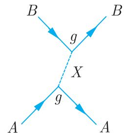
Figure 1.14 Contribution to the reaction A + B \rightarrow A + B from the exchange of a particle X .
