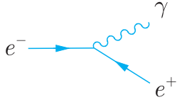
Figure 1.6 The forbidden vertex e^- \rightarrow e^+ + \gamma .
