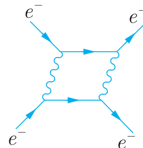
Figure 1.8 A contribution to electron–electron scattering from two-photon exchange.
