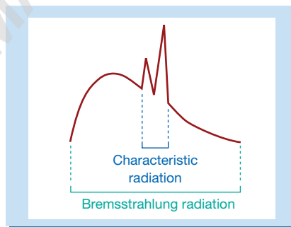
Figure 1.4 The X-ray spectrum
