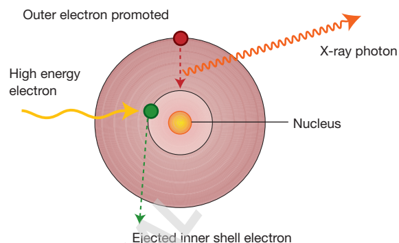
Figure 1.2 Characteristic radiation generation
