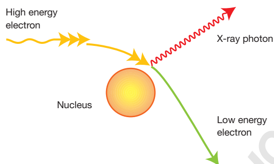
Figure 1.3 Bremsstrahlung radiation
