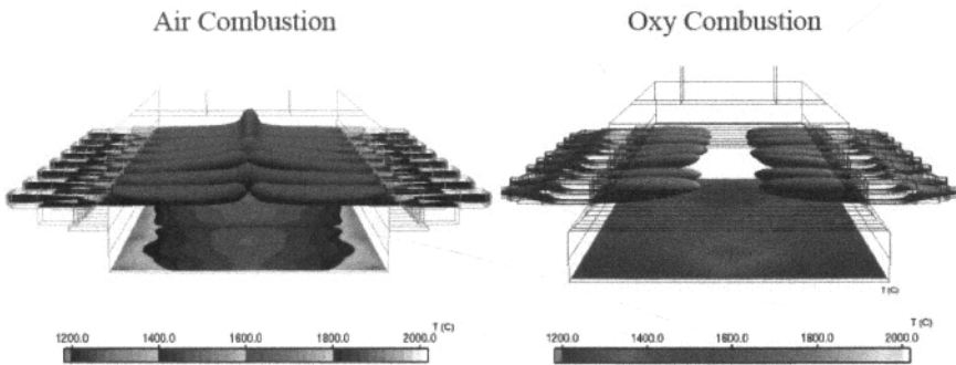
Figure 9: Modeling of face-to-face burners in one part of the zone downstream of the melter exit – for borosilicate container glass process: air combustion case (left side) and oxy combustion case (right side)
