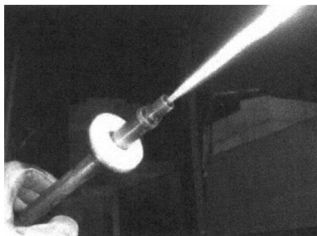
Figure 11: Picture of one ALGLASS FH burner operated outside the borosilicate container glass forehearth line
