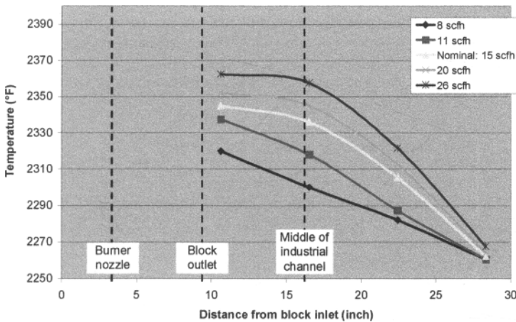
Figure 7: Graphic – Tests in the AIR LIQUIDE pilot tests – Temperature profile on chamber bottom when the ALGLASS FH burner was operated at five different powers inside the customer’s refractory block – for E glass fiber process
