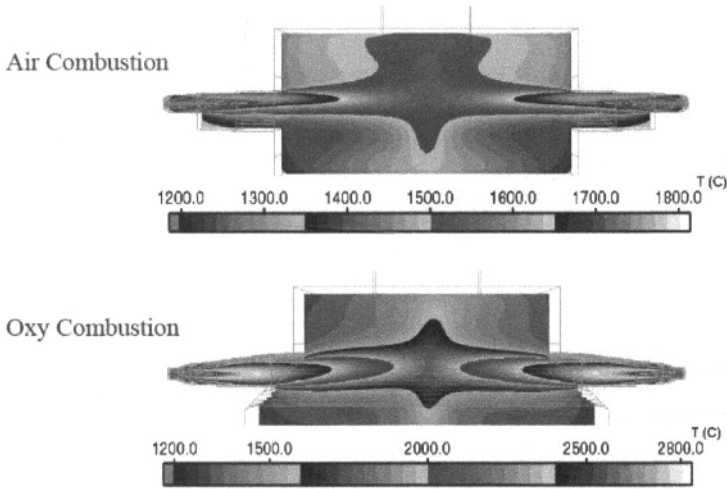
Figure 8: Modeling of two face-to-face burners in the zone downstream of the melter exit – for borosilicate container glass process: air combustion case (top) and oxy combustion case (bottom)
