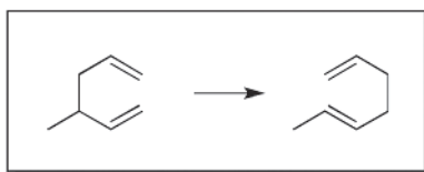
Scheme 1.6 Illustration of a concerted reaction (Cope rearrangement).
