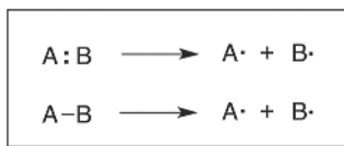
Scheme 1.4 Illustration of homolytic cleavage.
