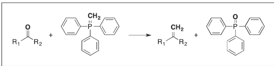
Scheme 1.1 Example of the Wittig reaction.
