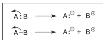
Scheme 1.9 Application of arrow-pushing to heterolytic cleavage using double-barbed arrows.
