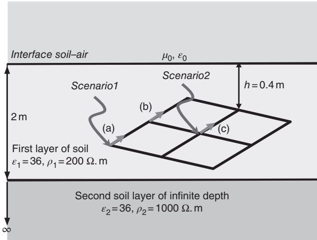
Figure 1.7 Horizontal grounding grid in two-layer soil.
