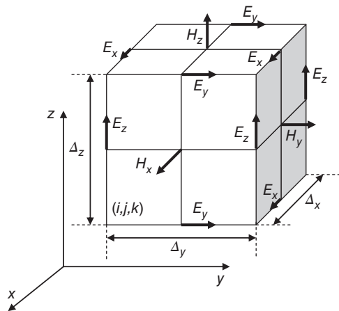
Figure 1.3 Configuration of electric and magnetic fields in a cell.
