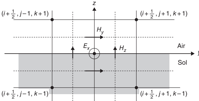
Figure 1.4 Treatment of the air-ground interface by the “the contour integral approach” method.
