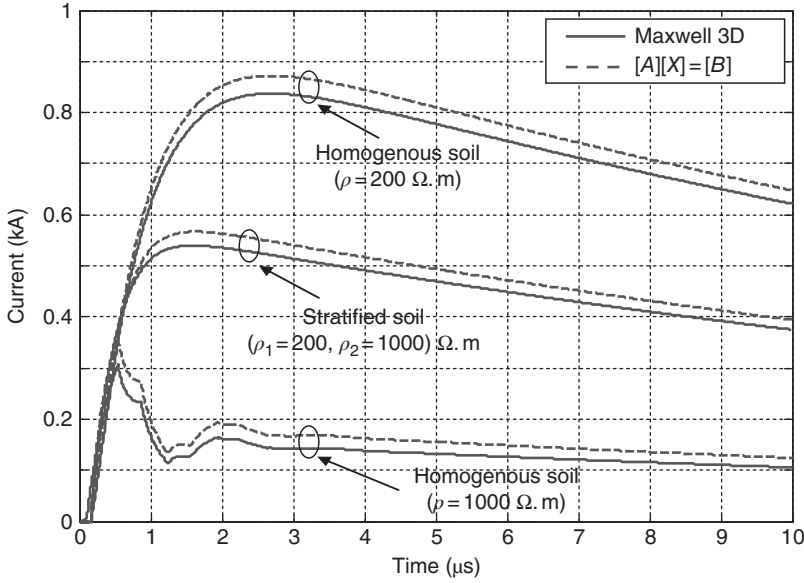
Figure 1.6 Transient current induced at the middle of the buried electrode.
