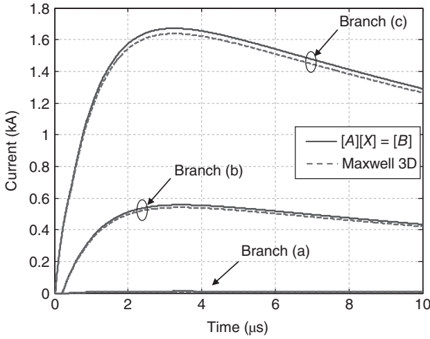
Figure 1.9 Transient currents induced at different points for the horizontal grounding grid (Scenario 2).
