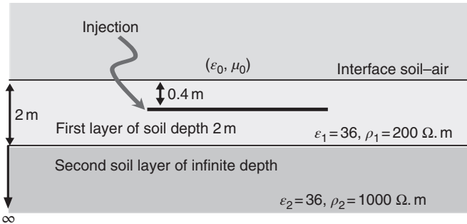
Figure 1.5 Horizontal grounding electrode in two-layer soil.
