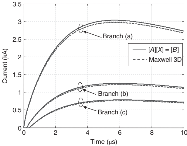
Figure 1.8 Transient currents induced at different points for the horizontal grounding grid (Scenario 1).
