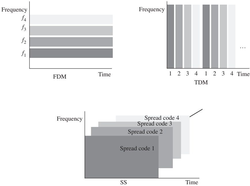
Figure 1.16 Media Sharing Schemes.
