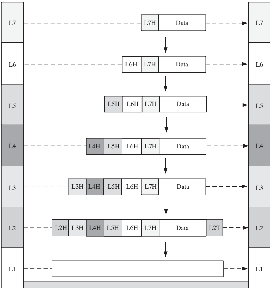
Figure 1.18 Composite Frame Construction Process.
