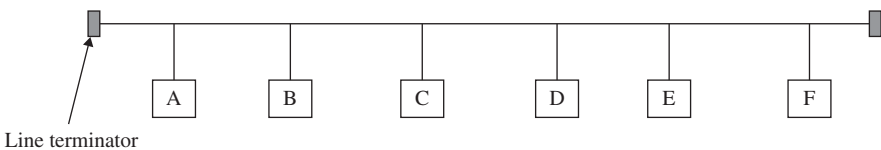
Figure 1.11 Bus Topology.
