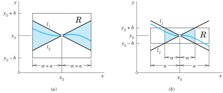
Fig. 27. The condition (2) of the existence theorem. (a) First case. (b) Second case
