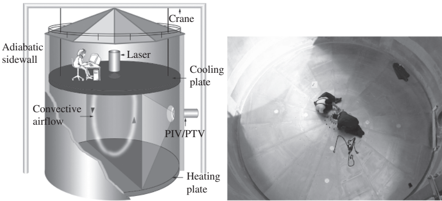
Figure 1.2 The experiment for studying thermal convection at the Ilmenau University of Technology, Germany. Turbulent convection similar to the convection observed in the atmosphere of Earth or Sun is simulated by air motion within a large barrel with thermally insulated walls and uniformly heated bottom. Source: Courtesy of André Thess.
