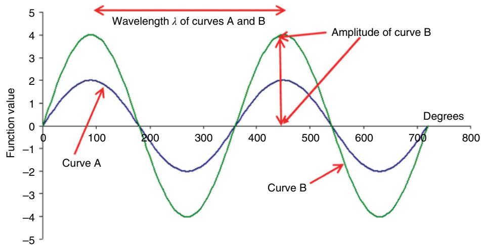
Figure 1.8 Two curves (waveforms) A and B have the same wavelength ( 360^\circ or 2\pi radians, x-axis). However, curve A has an amplitude of two units (y-axis), while curve B has an amplitude of four units. If we imagine that the two curves repeat to infinity and are moving to the right, like traces on an oscilloscope, then the frequency is the number of waveforms ( 0-2\pi ) that pass a fixed point in unit time (usually measured in cycles per second or Hertz, Hz). The period of the waveform is the time taken for one full waveform to pass a fixed point. These two waveforms have the same wavelength, frequency, and period and differ only in terms of their amplitude.
