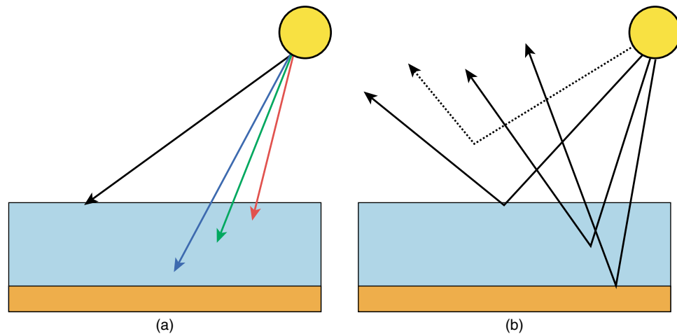
Figure 1.24 (a) Showing the differential penetration depths of red, green, and blue light in clear, calm water. The black line shows longer (infrared) wavelengths that are totally absorbed by the first few centimetres of water. (b) The solid arrows show, from right to left, bottom reflectance (the water depth is assumed to be less than the depth of penetration of blue light), volume reflectance (caused by light being scattered by suspended sediment particles, phytoplankton, and dissolved organic matter), and surface reflectance. The dotted line shows the path taken by light from the sun that interacts with the atmosphere in the process of atmospheric scattering (Chapter 3). Electromagnetic radiation scattered by the atmosphere may be considerably greater in magnitude than that which is backscattered by surface reflectance, volume reflectance, and bottom reflectance.
