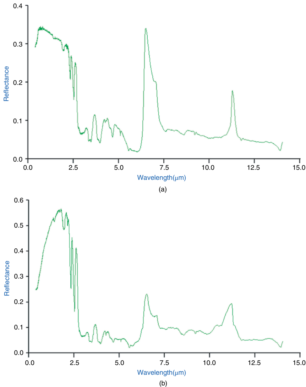
Figure 1.23 Reflectance and emittance spectra of (a) limestone and (b) basalt samples. Source: Data from the ASTER spectral library through the courtesy of NASA/Jet Propulsion Laboratory, California Institute of Technology, Pasadena, California, © California Institute of Technology. All rights reserved.
