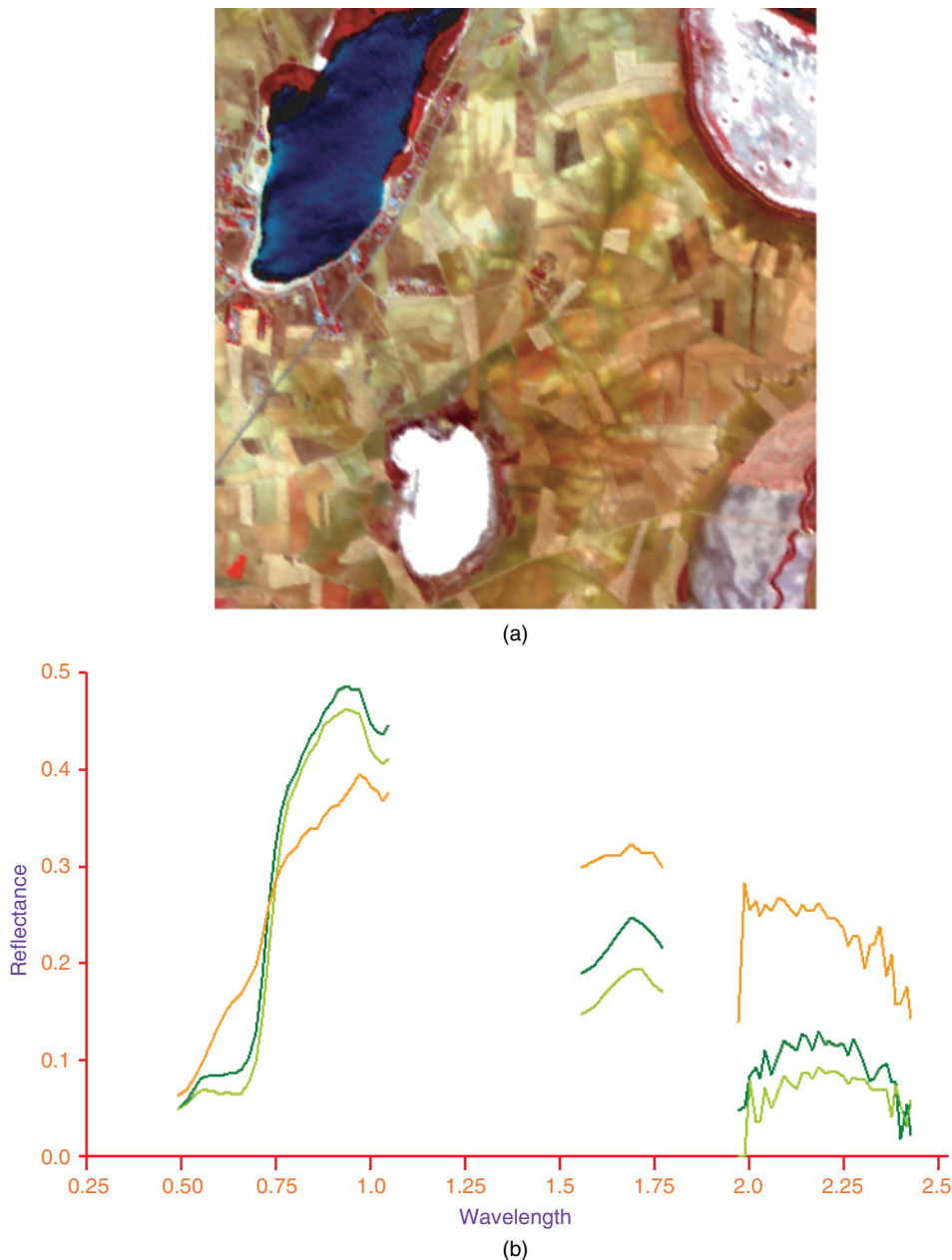
Figure 1.21 (a) DAIS image of part of La Mancha, Central Spain. (b) Reflectance spectra in the optical wavebands of three vegetation pixels selected from this image. The two green curves represent the typical spectral reflectance curves of active vegetation. The 2 pixels that these curves represent were selected from the bright red area in the bottom left of image (a) and the similar area by the side of the black lagoon. The third reflectance curve, shown in orange, was selected from the orange area in the top right of image (a). The spectral reflectance plots are discontinuous because parts of the atmosphere absorb and/or scatter incoming and outgoing radiation (see Figure 1.7 and Chapter 3). DAIS image source: German Space Agency, DLR.
