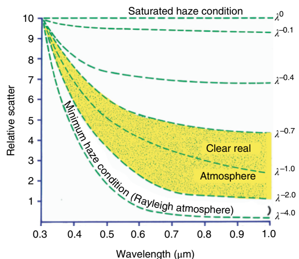
Figure 1.18 Relative scatter as a function of wavelength for a range of atmospheric haze conditions.
