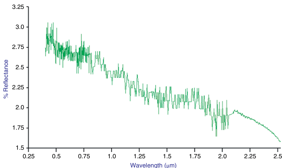
Figure 1.26 Reflectance spectrum of tap water from 0.4 to 2.55\ \mu\text{m} . Source: Data from the ASTER spectral library through the courtesy of NASA/Jet Propulsion Laboratory, California Institute of Technology, Pasadena, California, © California Institute of Technology. All rights reserved.
