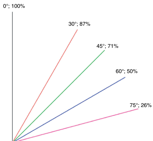
Figure 1.20 Lambert's Cosine Law. Assume that the illumination angle is 0°. A range of view angles is shown, together with the percentage of incoming radiance that is scattered in the direction of the view angle.
