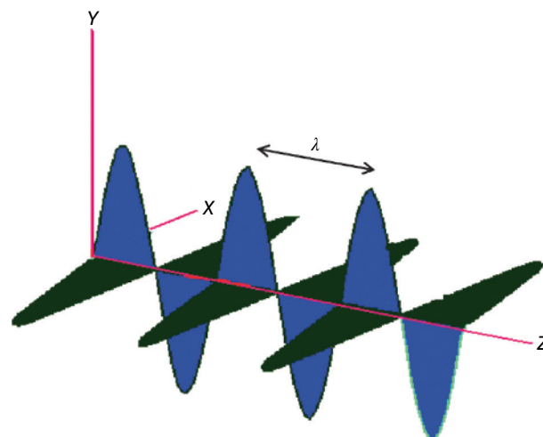
Figure 1.3 Electromagnetic wave. The wavelength of the electromagnetic energy is represented by the Greek letter lambda ( \lambda ). Source: Adapted from a figure by Nick Strobel, from http://www.astronomynotes.com/light/s2.htm . Accessed 5 January 2020.
