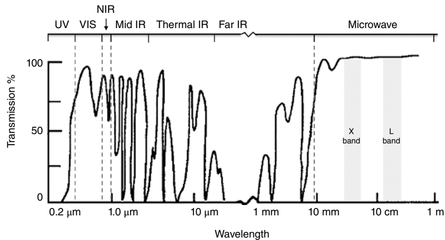
Figure 1.7 The electromagnetic spectrum showing the range of wavelengths between 0.2\mu\text{m} and 1\text{m} . The vertical dashed lines show the boundaries of wavebands such as ultraviolet (UV) and near-infrared (NIR). The shaded areas between 2 and 35\text{cm} wavelength indicate two microwave wavebands (X band and L band) that are used by imaging radars. The curve shows atmospheric transmission. Areas of the electromagnetic spectrum with a high transmittance are known as atmospheric windows. Areas of low transmittance are opaque (due to scattering/absorption losses) and cannot be used to remotely sense the Earth's surface.
