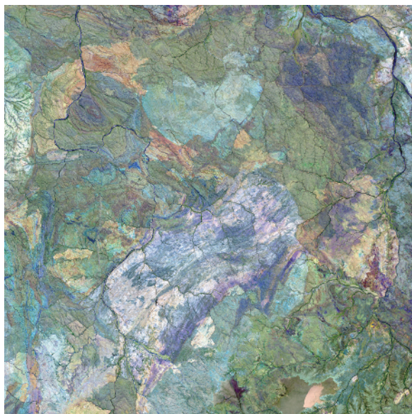
Figure 1.22 Landsat-7 Thematic Mapper image of the Great Sandy Desert of Western Australia. Despite its name, not all of the desert is sandy, and this image shows how the differing spectral reflectance properties of the weathered rock surfaces allow rock types to be differentiated. Field work would be necessary to identify the specific rock types, while comparison of the spectral reflectance properties at each pixel with library spectra (such as those contained in the ASTER spectral library, for example Figure 1.23) may allow the identification of specific minerals. The image was collected on 24 February 2001 and was made using shortwave infrared, near-infrared, and red wavelengths as the red, green, and blue components of this false colour composite image. Source: Image courtesy NASA/USGS/Public Domain.
