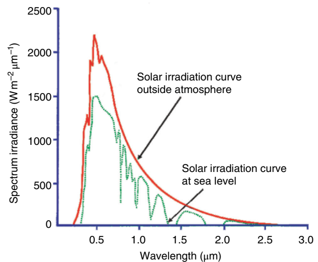
Figure 1.17 Solar irradiance at the top of the atmosphere (solid line) and at sea level (dotted line). Differences are due to atmospheric effects as discussed in the text. See also Figure 1.7.
