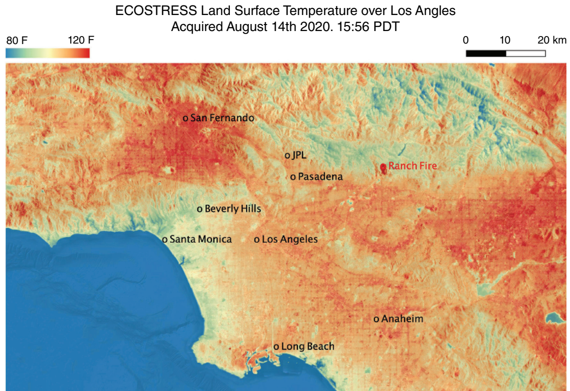
Figure 1.12 Land surface temperature map of Los Angeles County, California. This image was collected on 14 August 2020 by NASA's Ecosystem Spaceborne Thermal Radiometer Experiment on Space Station (ECOSTRESS), which measured a peak land surface temperature in the San Fernando Valley, northwest of downtown Los Angeles, of 128.3°F (53.5°C). ECOSTRESS has five bands in the thermal infrared region (8.29–12.09 \mu\text{m} ), which can be used to measure and monitor heat-related phenomena like heatwaves, fires, and volcanoes. Source: Image courtesy NASA/JPL/Public Domain.
