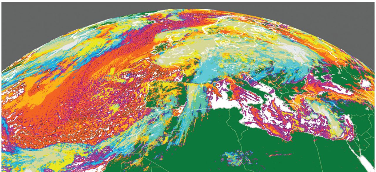
Figure 1.13 Portion of a Meteosat-11 visible channel image of Europe and North Africa taken on the morning of 21 October 2020. The colour palette indicates cloud type and characteristics. These cloud type products are essential for the generation of the cloud top temperature and height product, cloud microphysics, and for the identification of precipitation clouds. Source: Image courtesy EUMETSAT 2020.
