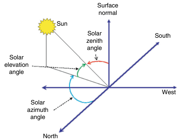
Figure 1.19 Solar elevation and azimuth angles. The elevation angle of the sun – target line is measured upwards from the horizontal plane. The zenith angle is measured from the surface normal and is equal to (90^\circ - \text{elevation angle})^\circ . Azimuth is measured clockwise from north.
