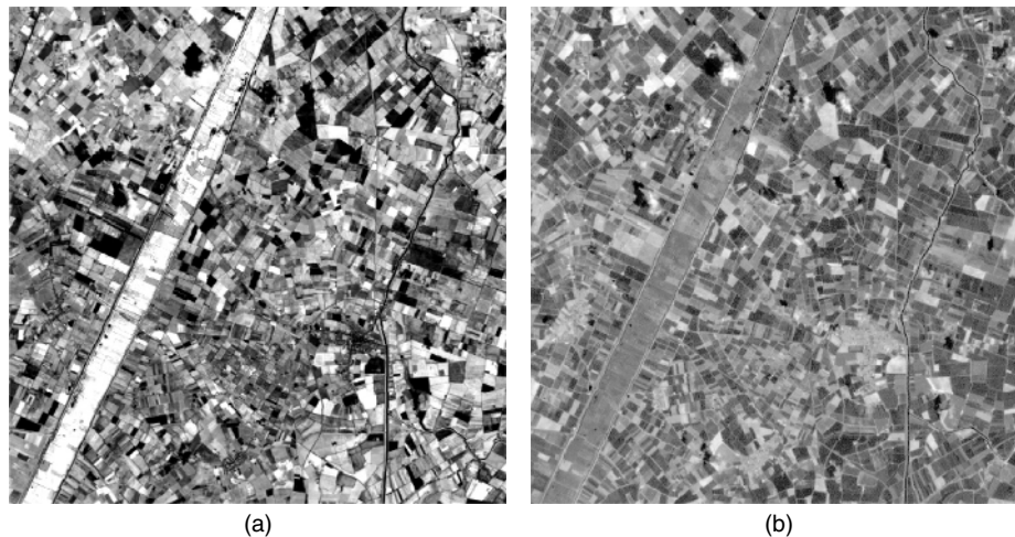
Figure 1.11 Image of ground reflectance in (a) the 0.75–0.90 \mu\text{m} band (near-infrared) and (b) the middle infrared (2.08–2.35 \mu\text{m} ) image of the same area as that shown in Figure 1.10. These images were collected by the Landsat-5 Thematic Mapper (bands 4 and 7). Source: Image courtesy NASA/USGS/Public Domain.
