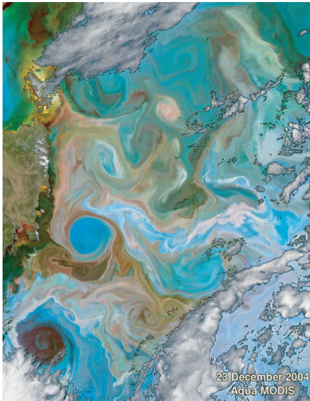
Figure 1.27 This image of the ocean east of Tasmania in December 2004 depicts subtle differences in water colour that result from varying distributions of such scattering and absorbing agents in the water column as phytoplankton, dissolved organic matter, suspended sediment, bubbles, and so on. The ocean colours shown above result from independently scaling the satellite-derived normalised water-leaving radiances (nLw) at 551, 488, and 412 nm and using the results as the red, green, and blue components of the image, respectively. Differences in the colours may also partially reflect differences in atmospheric components or levels of sunglint and sky glint or differences in the path that light takes through the MODIS instrument. The MODIS instrument is described in Section 2.3. Source: Image courtesy NASA/USGS/Public Domain.
