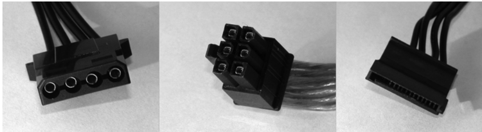
FIGURE 1.34 Peripheral power connectors
