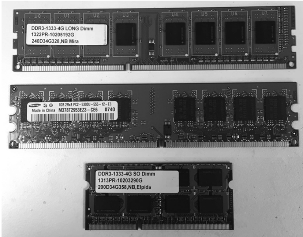
FIGURE 1.19 Memory module form factors
