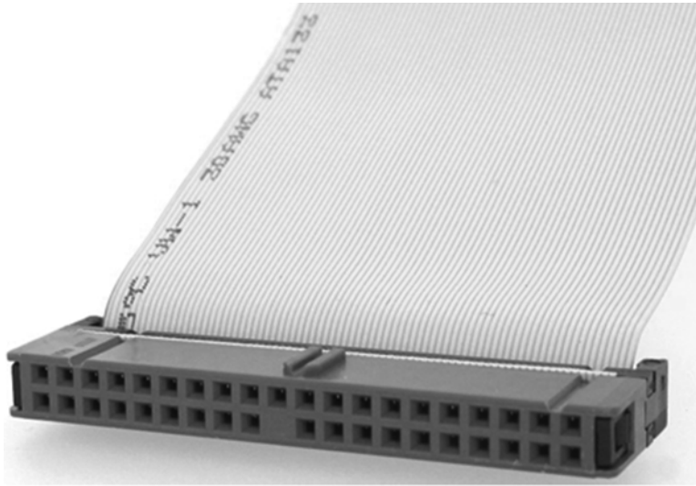
FIGURE 1.22 PATA and SATA data cables
