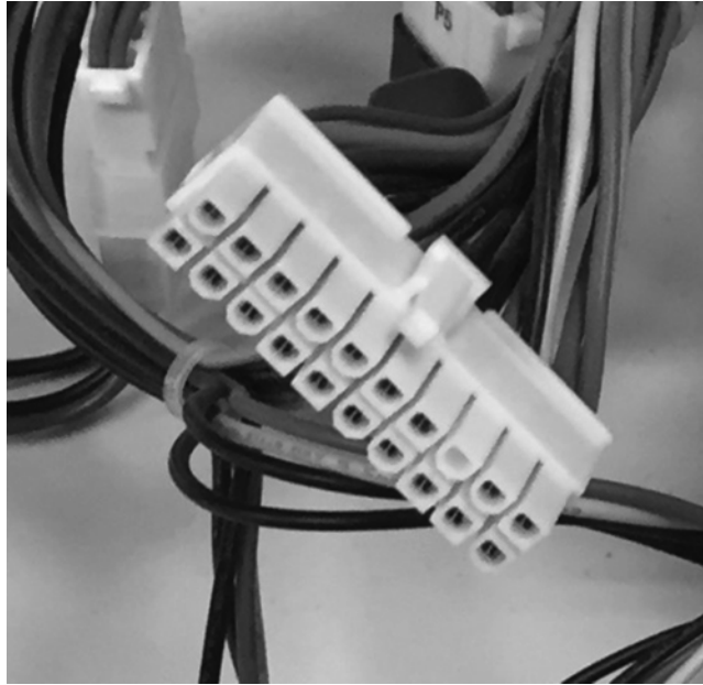
FIGURE 1.33 A 20-pin ATX power connector
