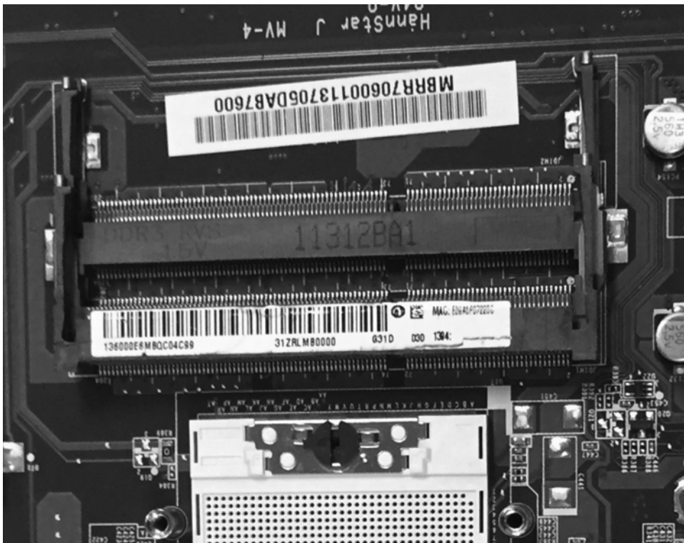
FIGURE 1.5 SODIMM slots
