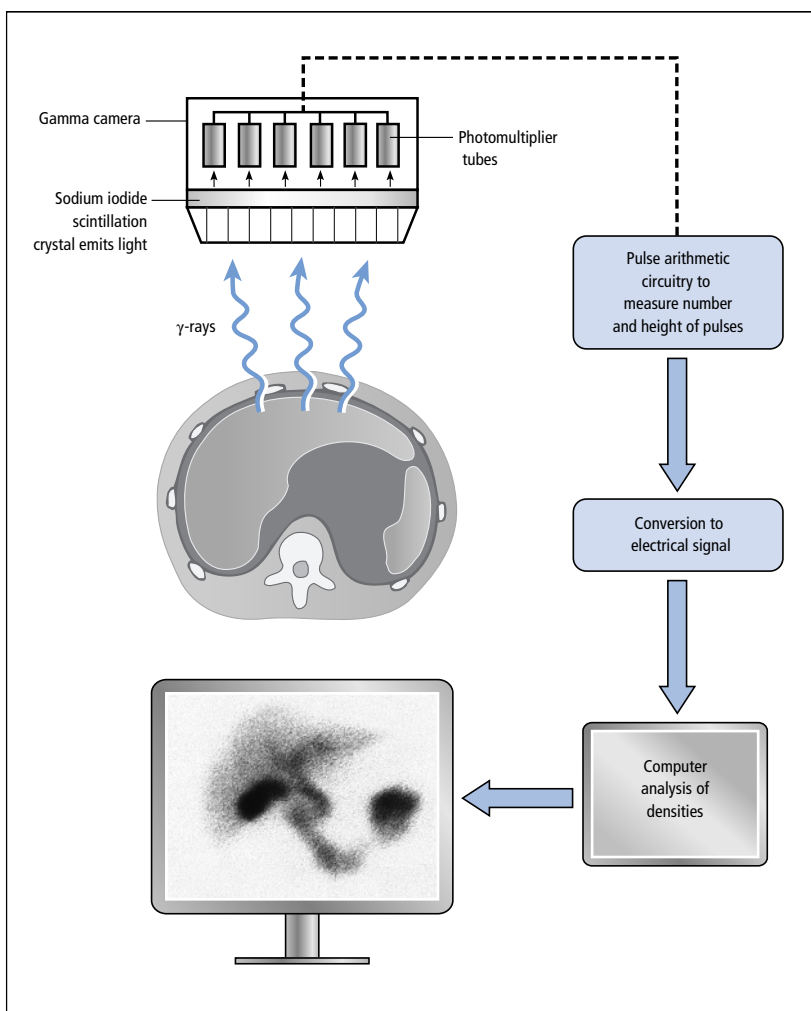
Figure 1.9 Basic principles of isotope scanning.
