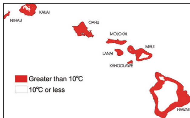
FIGURE 1.26D Average February minimum temperature.
