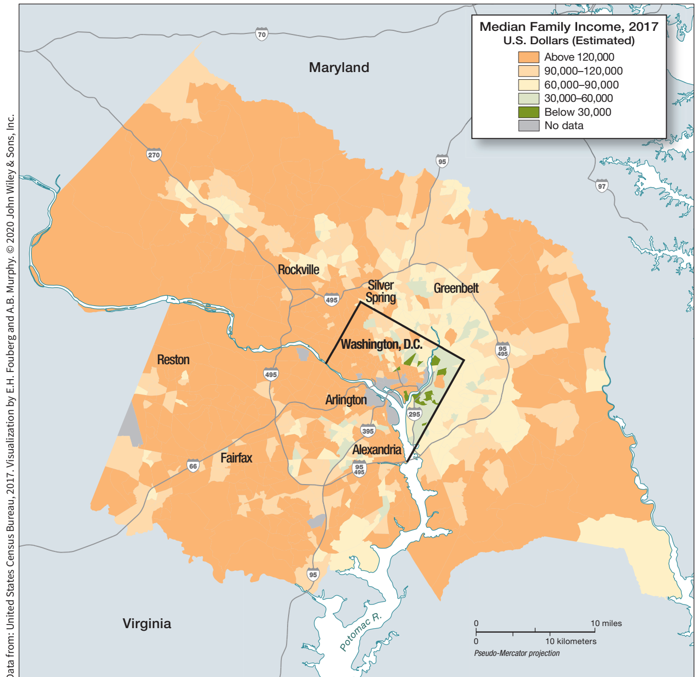
FIGURE 1.20 Median Family Income (in U.S. Dollars) in Washington, DC. Washington, D.C. is a diamond shape with the Potomac River as its southwest border in the middle of the map. Notice the sharp contrast in income between western and eastern D.C. The surrounding suburbs in Maryland and Virginia are also mapped with the same general trend: The western suburbs have higher incomes than the eastern suburbs.
