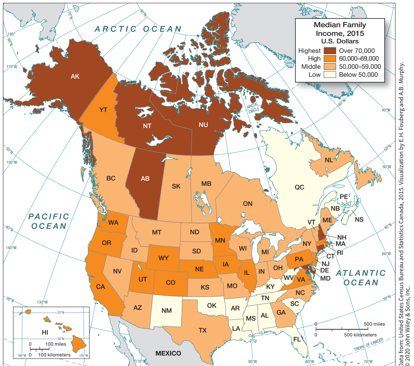
FIGURE 1.19 Median Family Income (in U.S. Dollars). The relatively higher incomes of Canadian provinces and the East Coast of the United States stand out. The relatively lower incomes of the American South also stand out on the map.
