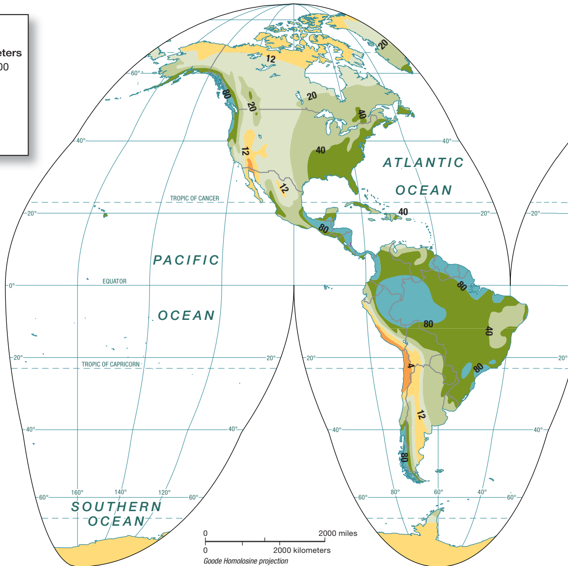
FIGURE 1.22 Average Annual Precipitation. This map shows the mean annual precipitation received around the world. The pattern on the map shows high precipitation along the equator, where consistent heating from the sun over the year means more incoming solar radiation is absorbed and released as warm air. When warm, moist air rises and reaches its dew point, condensation and precipitation follow. The rainforest climates are found along the equator. Locations that receive little precipitation are deserts, which are found in areas of Earth dominated by high-pressure cells. In a high-pressure cell, air descends from aloft to the ground and then goes outward, making it impossible for warm air to rise. Deserts receive rain when storms pass through them, not from the solar radiation they receive each day.
