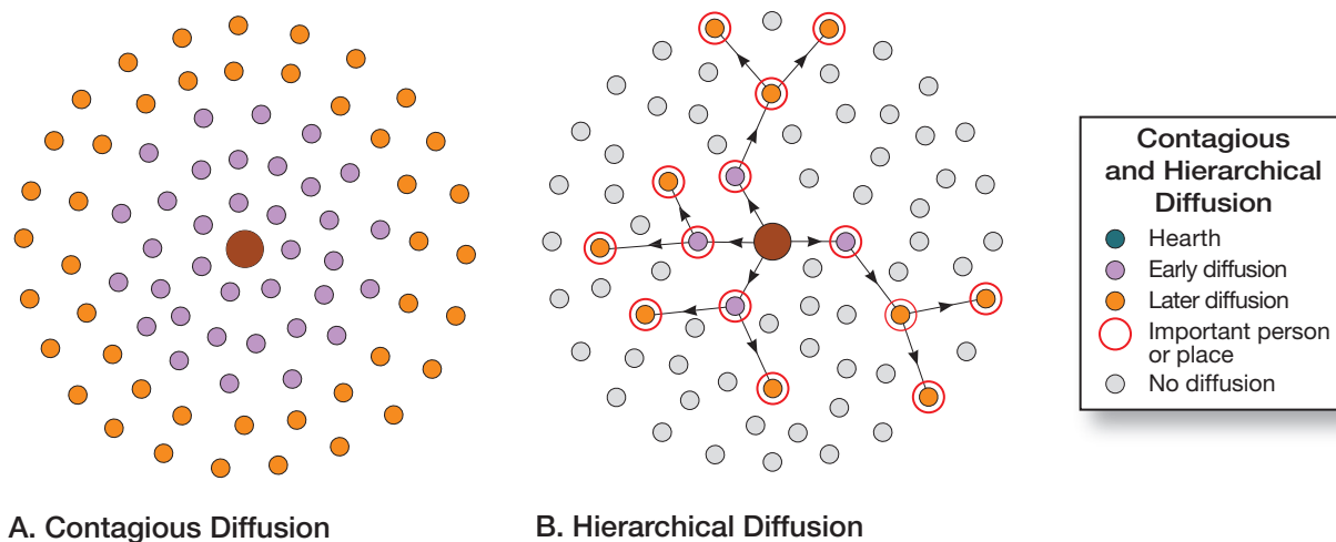
FIGURE 1.13 Contagious and Hierarchical Diffusion. In contagious diffusion, the trait spreads from the hearth outward contiguously and evenly. In hierarchical diffusion, the trait spreads from the hearth to the most linked or most important people or places first.
