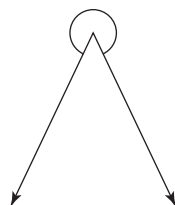
Reflex angle
