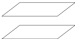
Parallel planes
