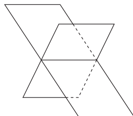
Intersecting planes
