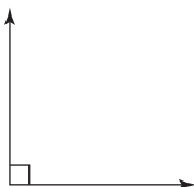
Right angle
