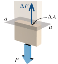
FIGURE 1.1c Stress at a point.
