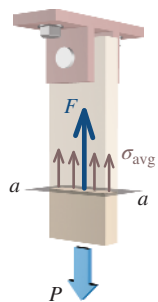
FIGURE 1.1b Average stress.
