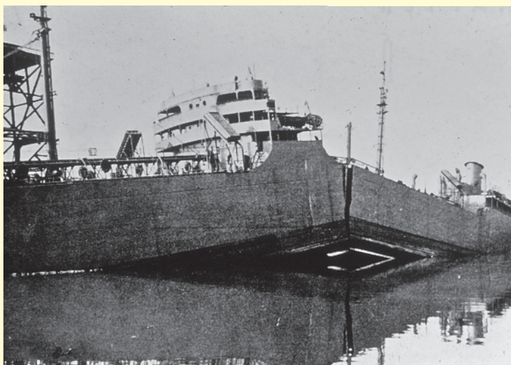
Figure 1.3 In January 1943, the T2 tanker Schenectady fractured in two amidships, after having completing sea trials and while moored at dock in Portland, Oregon, USA. At the time of failure, the seawater temperature was 4°C and the winds were light. This event was catastrophic and very loud—it was heard as far as a mile away. The fracture extended through the deck, sides of the hull, longitudinal bulkheads, and bottom girders. Consequently, the ship jack-knifed as the central region of the ship rose completely out of the water.
