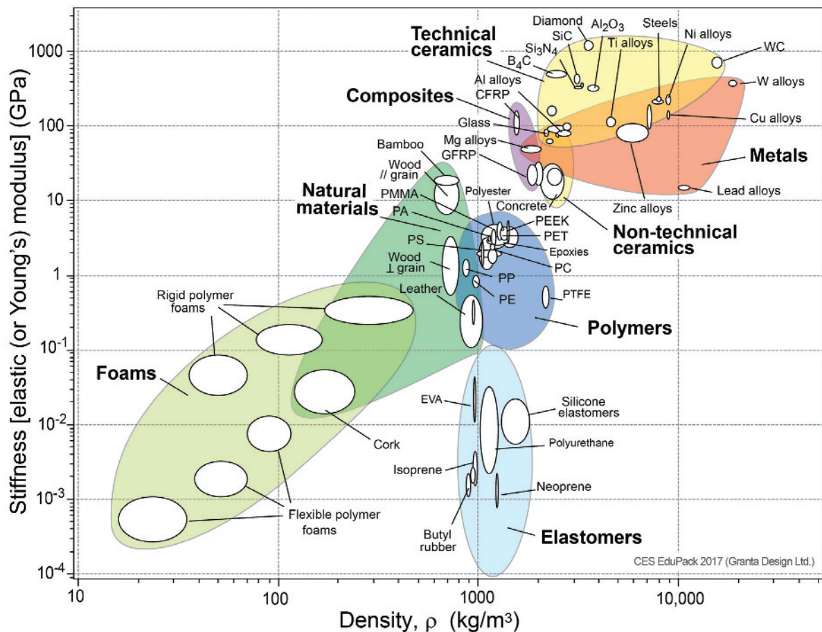
Figure 1.12 Modulus of elasticity (stiffness) versus density materials selection chart. (Based on CES EduPack 2017, Granta Design Ltd.)
