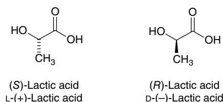
FIGURE 1.1 Two enantiomeric forms of lactic acid: (S)- and (R)-2-hydroxypropionic acid.
