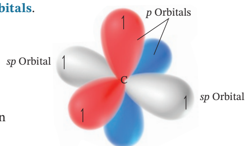
FIGURE 1.29 An sp -hybridized carbon atom.
