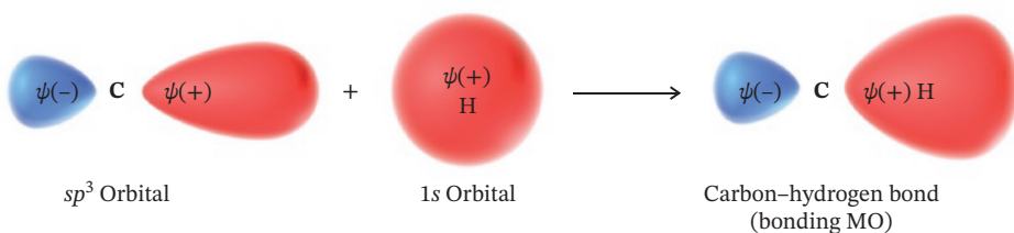
FIGURE 1.16 Formation of a C—H bond.
