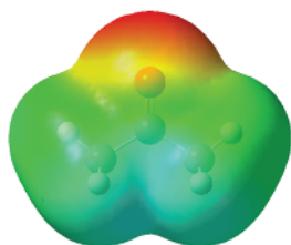
FIGURE 1.5 An electrostatic potential map for acetone. Regions of higher electron density trend toward red and regions of lower electron density trend toward blue.
