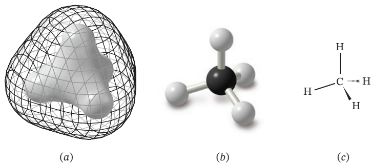
FIGURE 1.18 (a) In this structure of methane, based on quantum mechanical calculations, the inner solid surface represents a region of high electron density. High electron density is found in each bonding region. The outer mesh surface represents approximately the furthest extent of overall electron density for the molecule. (b) This ball-and-stick model of methane is like the kind you might build with a molecular model kit. (c) This structure is how you would draw methane. Ordinary lines are used to show the two bonds that are in the plane of the paper, a solid wedge is used to show the bond that is in front of the paper, and a dashed wedge is used to show the bond that is behind the plane of the paper.
