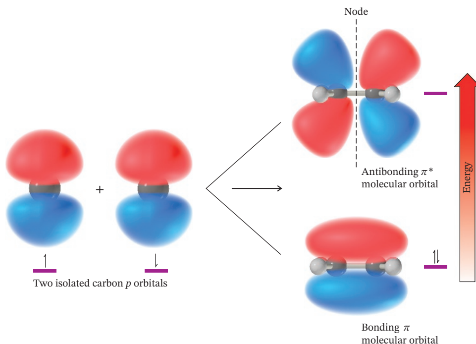
FIGURE 1.26 How two isolated carbon p orbitals combine to form two \pi (pi) molecular orbitals. The bonding MO is of lower energy. The higher energy antibonding MO contains an additional node. Both orbitals have a node in the plane containing the C and H atoms.
