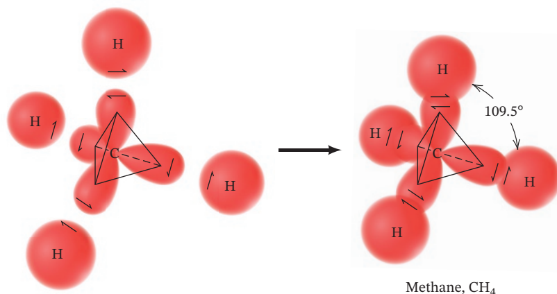
FIGURE 1.14 The hypothetical formation of methane from an sp^3 -hybridized carbon atom and four hydrogen atoms. In orbital hybridization, we combine orbitals, not electrons. The electrons can then be placed in the hybrid orbitals as necessary for bond formation but always in accordance with the Pauli principle of no more than two electrons (with opposite spin) in each orbital. In this illustration, we have placed one electron in each of the hybrid carbon orbitals. In addition, we have shown only the bonding molecular orbital of each C–H bond because these are the orbitals that contain the electrons in the lowest energy state of the molecule.
