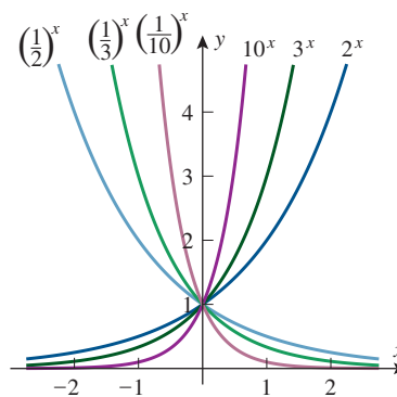
FIGURE 1.8.2 The family y = b^x ( b > 0 )
