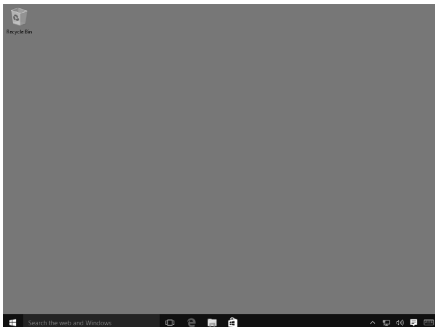
FIGURE 1.18 Windows 10 screen
