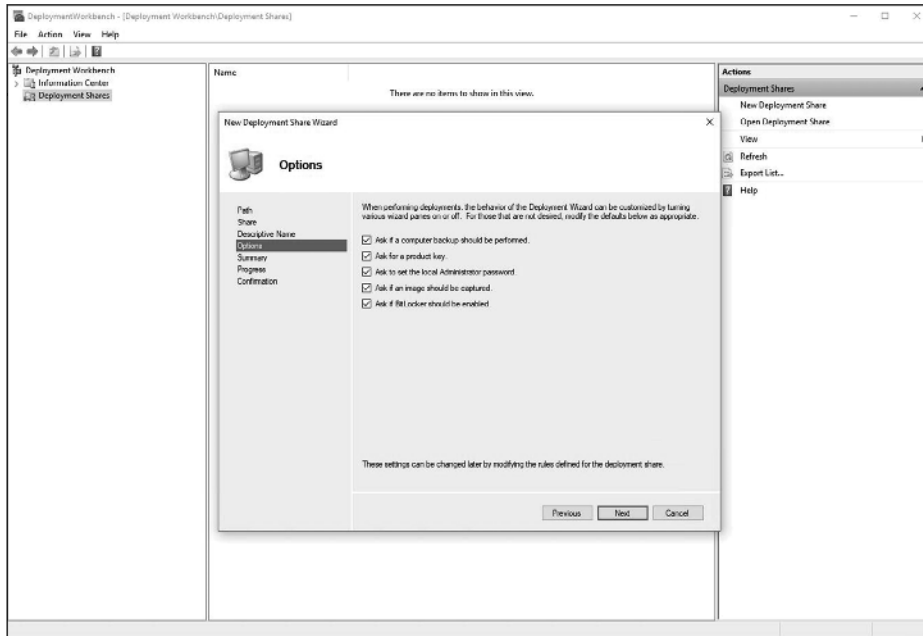
FIGURE 1.25 Options screen
