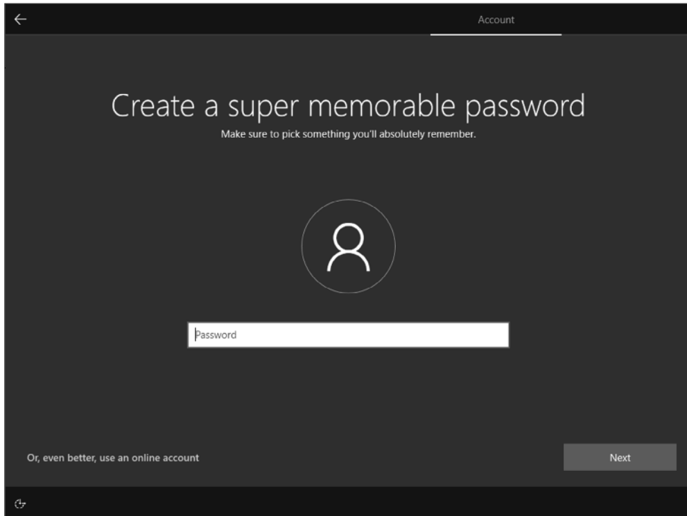
FIGURE 1.10 Windows 10 screen
