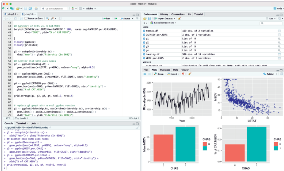
FIGURE 1.3 RSTUDIO SCREEN
