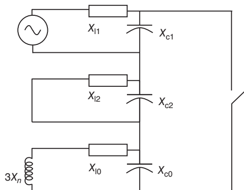
Figure 1.3 Symmetrical component representation for ground fault with grounding reactor.
