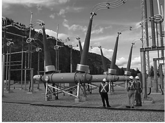
Figure 1.13 (a) Live-tank 345 kV SF 6 circuit breaker. Source: Courtesy of Appalachian Power Company. (b) Dead-tank 500 kV SF 6 circuit breaker.
