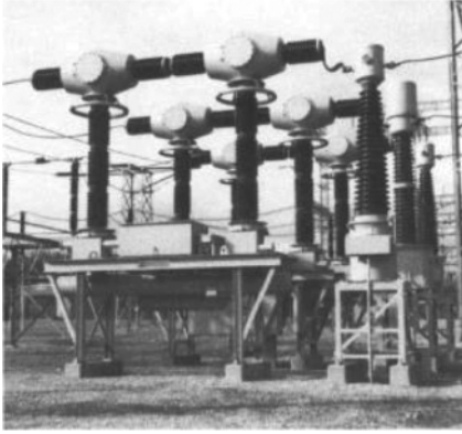
Figure 1.13 (a) Live-tank 345 kV SF 6 circuit breaker. Source: Courtesy of Appalachian Power Company. (b) Dead-tank 500 kV SF 6 circuit breaker.
