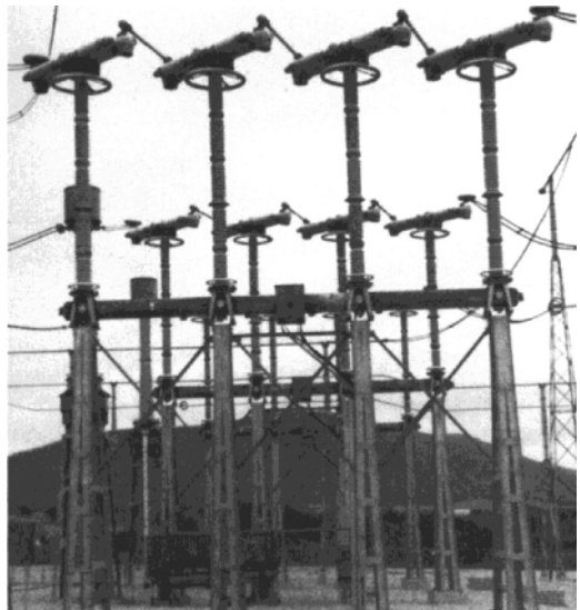
Figure 1.15 Live-tank, air-blast circuit breaker and a current transformer for 800 kV. Source: Courtesy of Appalachian Power Company.
