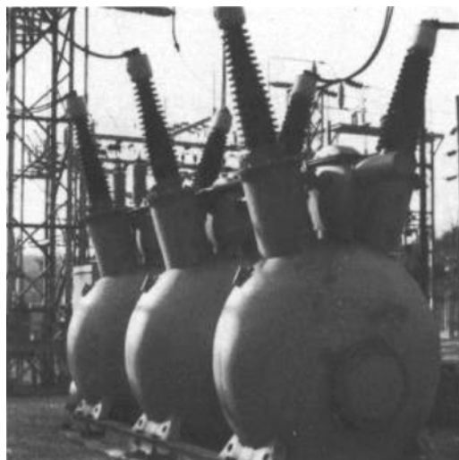
Figure 1.12 A 138 kV oil circuit breaker. Source: Courtesy of Appalachian Power Company.
