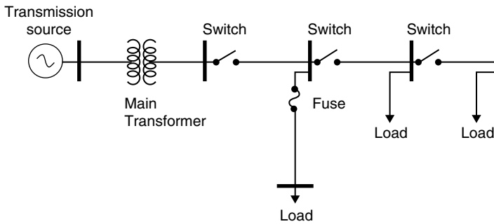
Figure 1.4 Radial power system.
