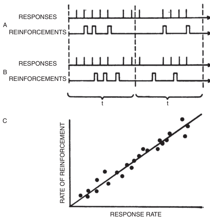
Figure 1.3 Contingency as correlation.
