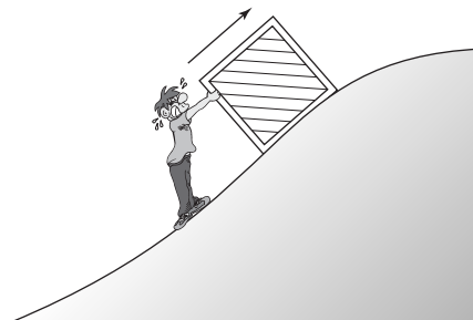
Calculus problem
