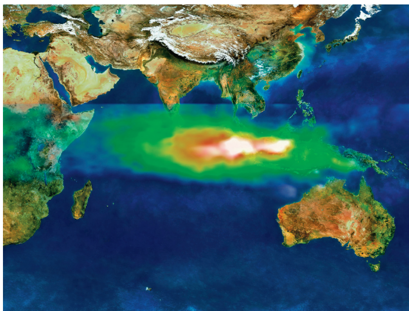
Figure 1.39 Aerosol emissions from fires in Indonesia, October 1997. White represents smoke near the fire and colours indicate smog being carried in to the Troposphere by high altitude winds. This was taken using NASA's Earth Probe Total Ozone Mapping Spectrometer (TOMS) satellite instrument ( http://visibleearth.nasa.gov ). NASA.
