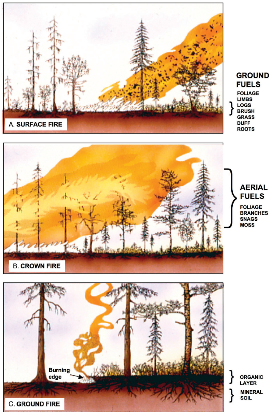
Figure 1.8 Types of wildfire and fuel sources. (From Scott, 2000, modified from Davis, 1959).
