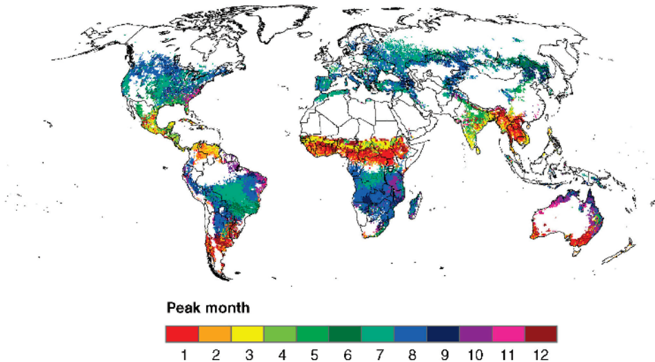
Figure 1.45 Simulating fire using the SPITFIRE model. These simulations can be matched with actual data (MODIS) to indicate the power of the model. (From Thonicke et al. , 2010).
