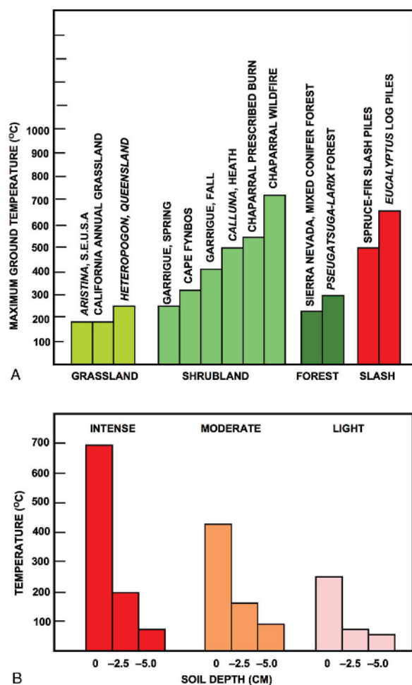
Figure 1.13 Ground temperature of fires.
