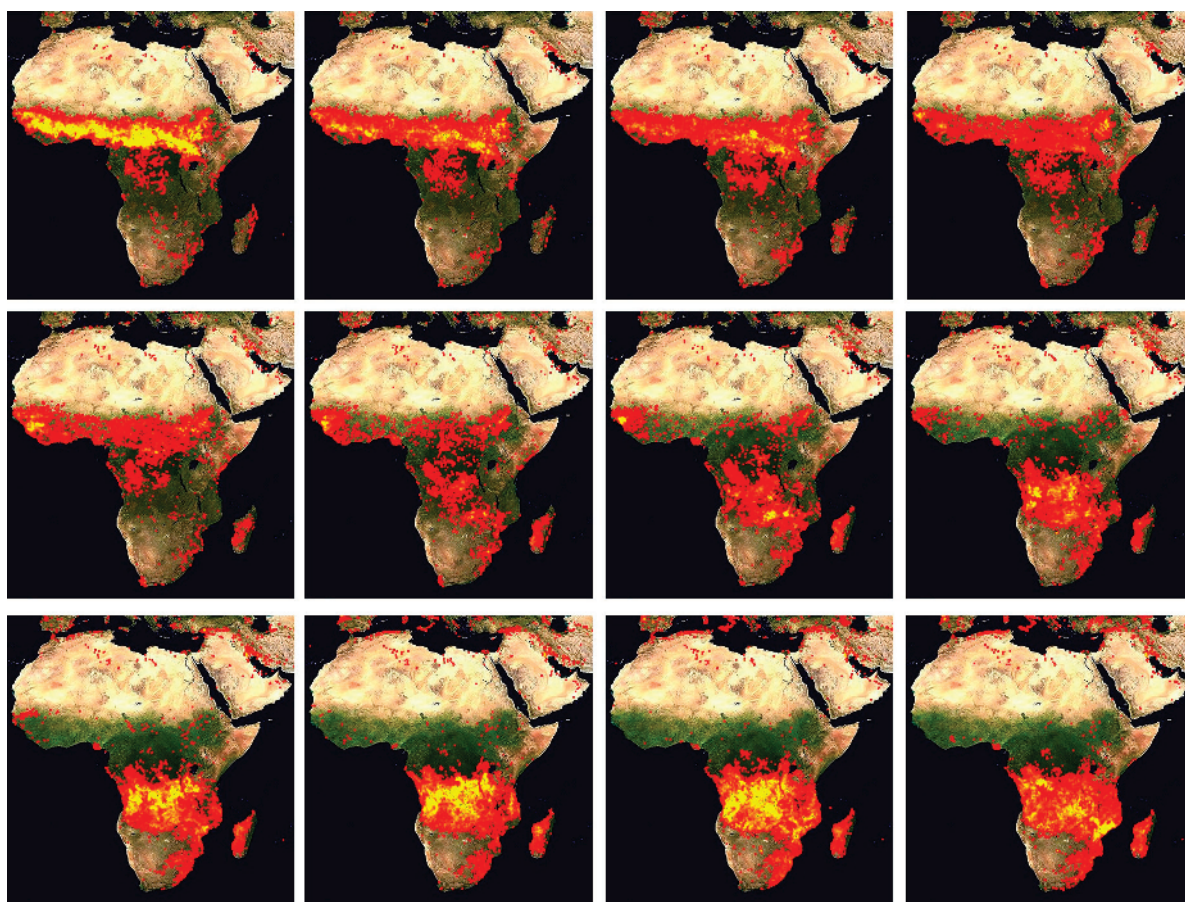
Figure 1.35 Variation of fire across Africa in 2005. Each image was processed from a ten-day period within a month from Jan to August (Jan 1–10; Jan 21–30; Feb 10–19; Mar 2–11; Mar 22–31; April 11–20; May 1–10; May 20–30; Jun 10–19; Jun 30–Jul 9; Jul 20–29; Aug 9–18). Successive images show the shift of fire through the year. Red indicates a single fire in an area over the period and yellow indicates more. These images were processed using data from MODIS on NASA's Terra and Aqua satellites. ( http://earthobservatory.nasa.gov ). NASA.
