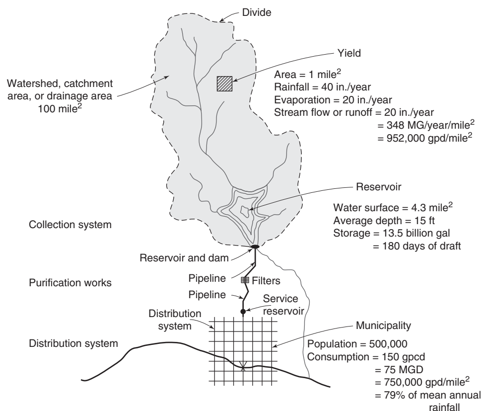
Figure 1.1 Rainfall, Runoff, Storage, and Draft Relations in the Development of Surface Water. Conversion factors: 1 mi 2 = 2.59 km 2 ; 1 in. /yr = 25.4 mm/yr; 1 ft = 0.3048 m; 1 MG/yr/mi 2 = 1.46 ML/yr/km 2 ; 1 gpd/mi 2 = 1.461 L/d/km 2 ; 1 billion gal = 1 BG = 3.785 billion L = 3.785 BL; 1 gpcd = 3.785 Lpcd; 1 MGD = 3.785 MLD.
