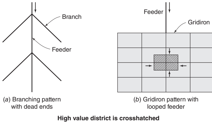
Figure 1.9 Patterns of Water Distribution Systems
