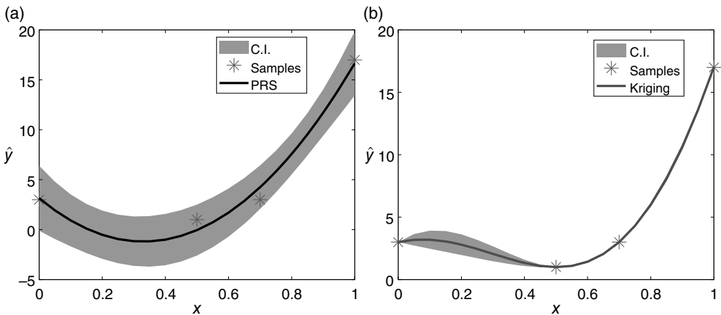
Figure 1.4 Polynomial response surface versus Kriging surrogate models. (a) Polynomial response surface and (b) Kriging surrogate.
