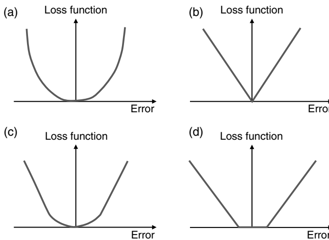
Figure 1.12 Loss functions. (a) Quadratic loss function ( L_2 -norm), (b) linear loss function ( L_1 -norm), (c) Huber loss function, and (d) \epsilon -loss function.
