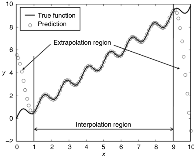
Figure 1.6 Fitting a function using a radial-basis neural network model in Matlab.
