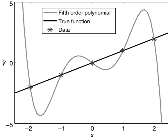
Figure 1.8 A surrogate model that is perfect at sample locations but has a large prediction error at unsampled locations.
