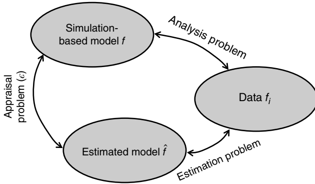
Figure 1.9 Overview of the surrogate modeling process.
