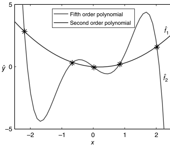
Figure 1.11 Different surrogate that fits the same samples.
