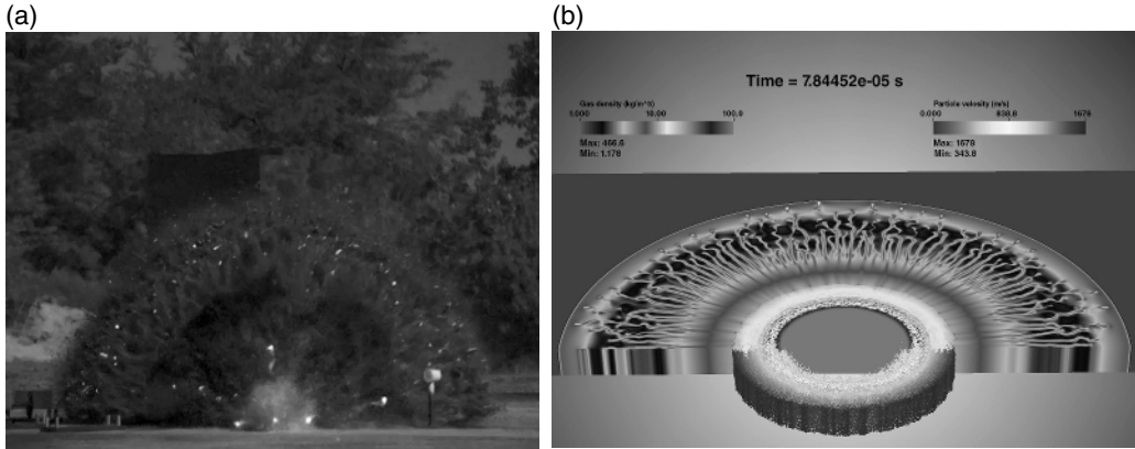
Figure 1.1 Experiment and simulation of dispersed multiphase flow: shock wave interaction with a particle bed. (a) Experiment at Eglin Air Force Base and (b) simulation at the University of Florida.
