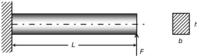
Figure 1.2 Bending of a cantilevered beam.
