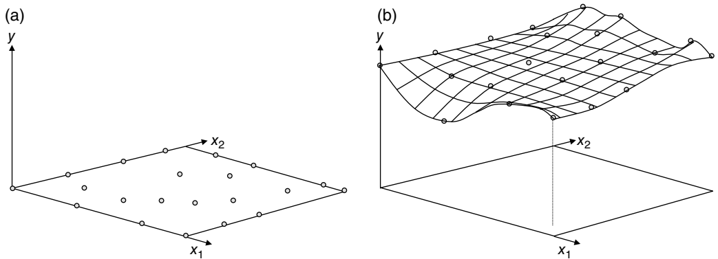
Figure 1.3 An example of samples in a 2D domain and the corresponding surrogate model. (a) Sample locations and (b) samples and fitted surrogate model.
