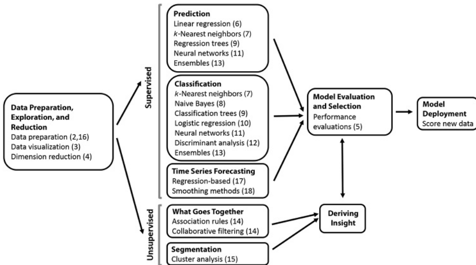
FIGURE 1.2 MACHINE LEARNING FROM A PROCESS PERSPECTIVE. NUMBERS IN PARENTHESES INDICATE CHAPTER NUMBERS
