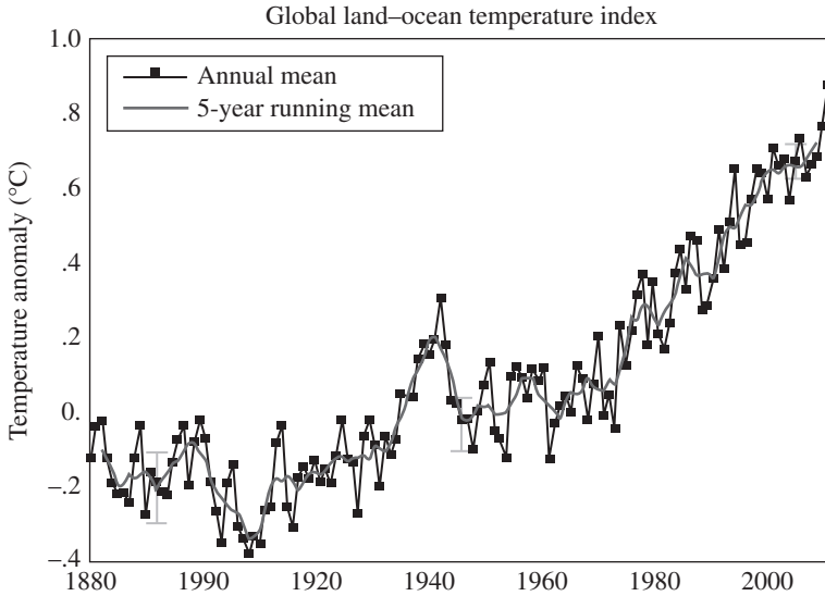
Figure 1.6 Global annual mean surface air temperature change. Source: Data from http://data.giss.nasa.gov/gistemp/graphs/ . Courtesy NASA.
