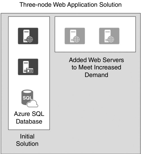
FIGURE 1.2 Horizontal scaling adds resources when they are needed and removes them when no longer needed.
