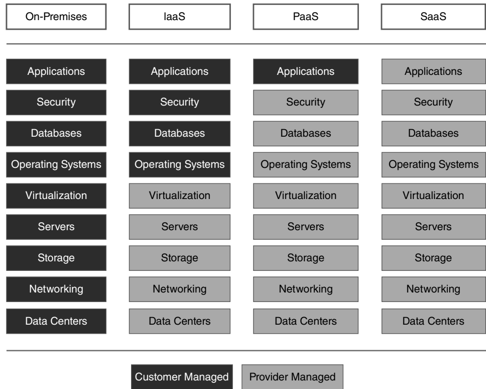
FIGURE 1.8 The three categories of Azure cloud computing have different levels of shared responsibility between your organization and Microsoft compared to the on-premises/self-hosted option.
