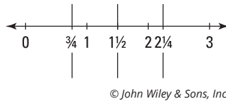
FIGURE 1-17: Fractions on the number line.
