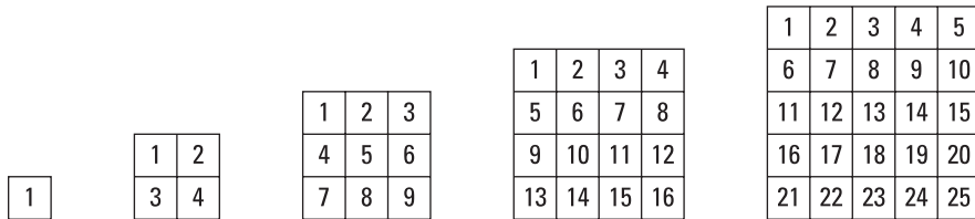
FIGURE 1-1: Square numbers for the numbers from 1 to 5.
