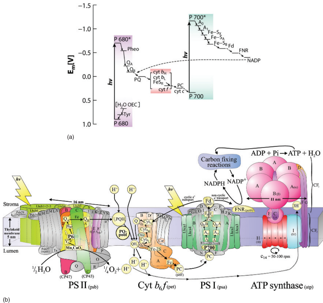
Figure 1.5 Schematic diagram of the noncyclic electron transfer pathway found in oxygenic photosynthetic organisms. The upper diagram (a) is an energetic picture of the electron transport pathway, incorporating the major reactions of photosynthesis into what is called the Z-scheme of photosynthesis. The lower diagram (b) is a spatial picture, showing the major protein complexes whose energetics are shown in the Z-scheme, and how they are arranged in the photosynthetic membrane. Neither view alone gives a complete picture, but together they summarize much information about photosynthetic energy storage. (a) Source: Hohmann-Marriott and Blankenship (2011). Reproduced with permission of Annual Reviews , and (b) Source: Figure courtesy of Dr. Jonathan Nield.
