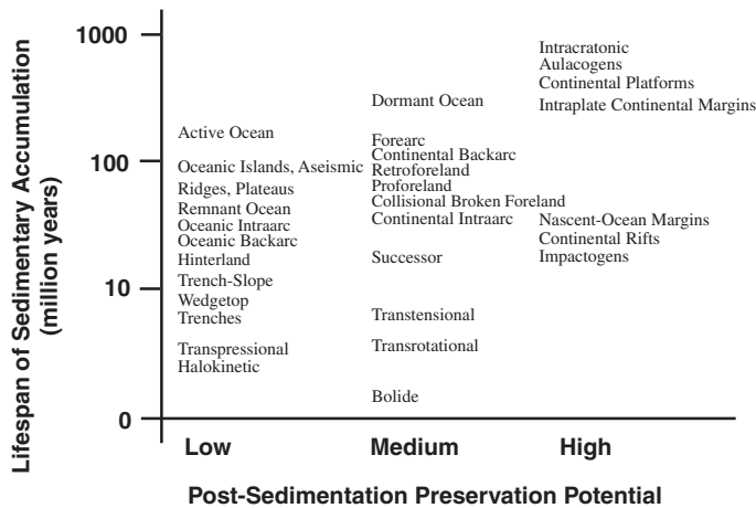
Fig. 1.2. Typical life spans for sedimentary basins versus their post-sedimentation preservation potential, which refers to average time interval during which basins will not be uplifted and eroded during and following sedimentation. Sedimentary or volcanic fill may be preserved as accretionary complexes during and after basin destruction (especially true for all strata deposited on oceanic crust). Intraplate continental margins have high preservation potential in the sense of retaining their basement, but are likely to be highly deformed and metamorphosed beneath and within suture belts, and may be difficult to recognize in ancient settings.
