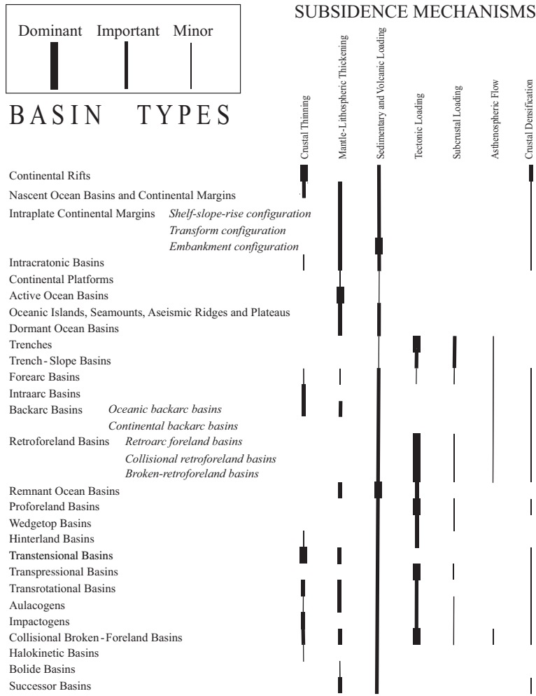
Fig. 1.1. Suggested subsidence mechanisms for all types of sedimentary basins.
