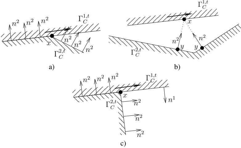
Figure 1.4. Example of discontinuity of the normal n^2 with respect to x : (a) when crossing an element boundary whether for projection or raytracing; (b) in the presence of concave boundaries for projection (in this case, even y is discontinuous); and (c) when raytracing fails (in this case, y becomes undefined)
