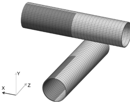
Figure 1.7. Geometry and mesh of hollow tubes in their undeformed configurations. For a color version of this figure, see www.iste.co.uk/lebon/mechanics.zip
