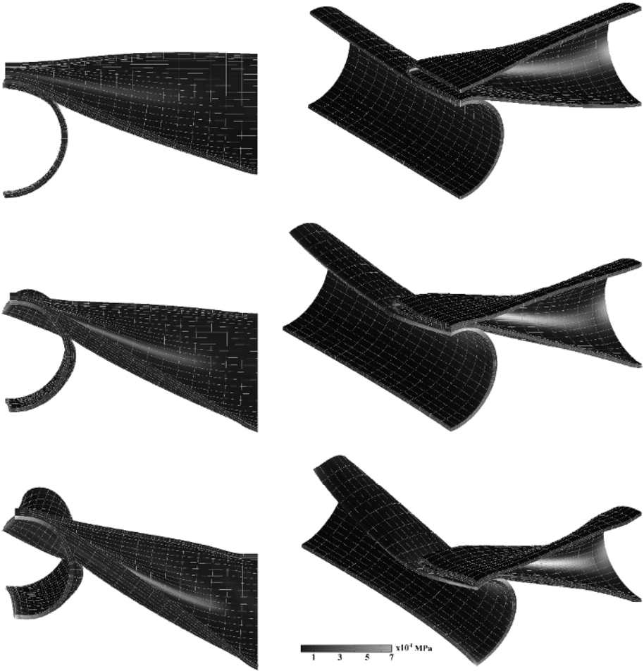
Figure 1.8. Von-Mises strain and stress of the two crossed tubes. Frictionless example for a penetration of 20 mm, 30 mm and 40 mm, respectively. For a color version of this figure, see www.iste.co.uk/lebon/mechanics.zip
