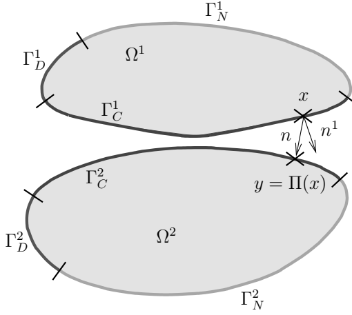
Figure 1.1. Two bodies with their respective potential contact boundaries. For a color version of this figure, see www.iste.co.uk/lebon/mechanics.zip
