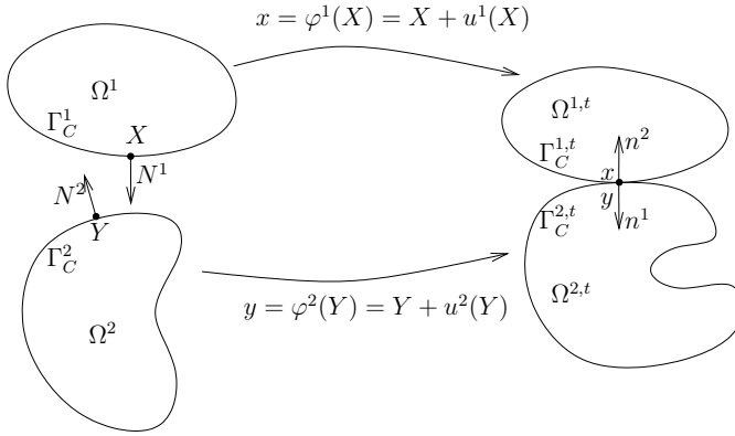
Figure 1.2. Large-strain Lagrangian description
