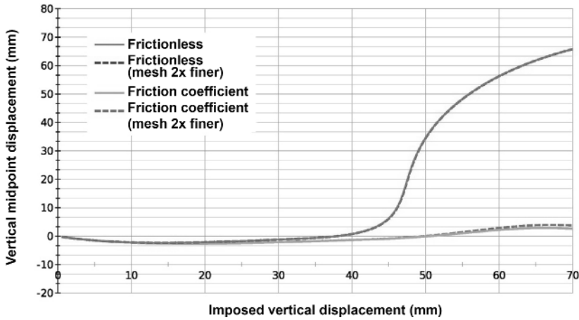
Figure 1.6. Vertical displacement of the half-ring midpoint for different mesh sizes. For a color version of this figure, see www.iste.co.uk/lebon/mechanics.zip
