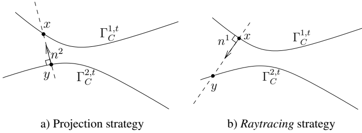
Figure 1.3. Illustration of projection and raytracing strategies
