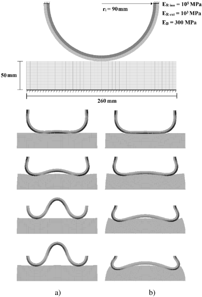
Figure 1.5. Deformation of the elastic half-ring coming into contact without (a) and with friction for \mathcal{F}=0.5 (b) for quadratic quadrilateral finite elements, at loading steps corresponding to 25, 45, 60 and 70 mm of penetration. For a color version of this figure, see www.iste.co.uk/lebon/mechanics.zip
