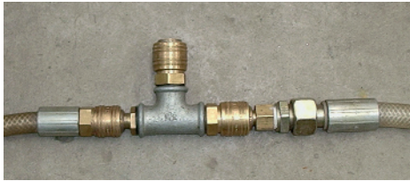
Fig. 1.4 Branch from the compressed air feed pipe to an individual lubrication point. (Source: Herrenknecht AG).
