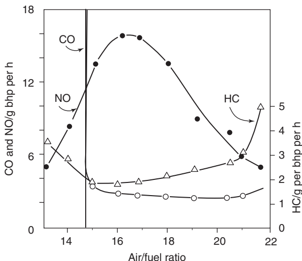
Figure 1.8 Effects of air/fuel ratio on the emission in auto-exhausts of hydrocarbon (HC), NO and CO (Hegedus and Gumbleton, 1980).
