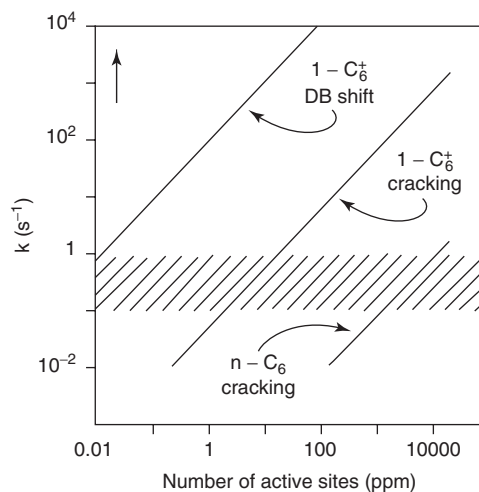
Figure 1.13 Plot of first-order rate coefficients versus concentration of active sites in ZSM-5 catalysts for the cracking of n -hexane ( n -C 6 ), for the cracking of 1-hexene (1-C 6 + ) and for the shift of double bond in 1-hexene (DB shift of 1-C 6 + ) (Haag, Lago and Weisz, 1984).
