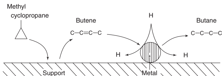
Figure 1.18 A bifunctional catalyst such as platinum on Al_2O_3 facilitates the isomerization of methylcyclopropane to 2-butene as well as the hydrogenation of 2-butene to butane. (After Boudart.)
